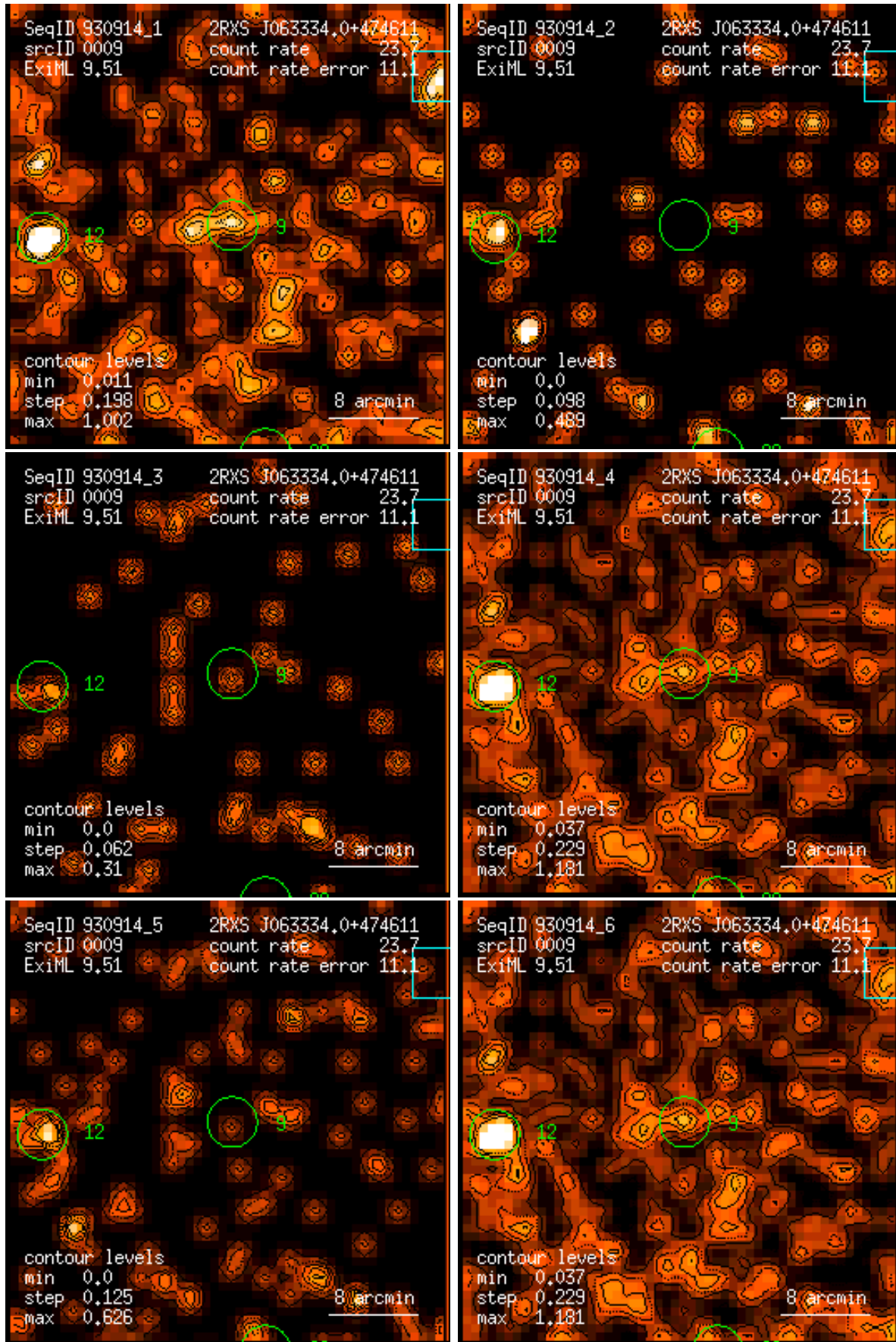
Figure 9: RASS 930914: detection 0009: band rate images, Gaussian filter: (1) PSPC channels 11 – 41, (2) 52 – 90, (3) 91 – 201, (4) 11 – 235, (5) 52 – 201, (6) 11 – 201. Broad band rates in counts/ks. Band rate contour levels in counts/ks/arcmin 2 .
