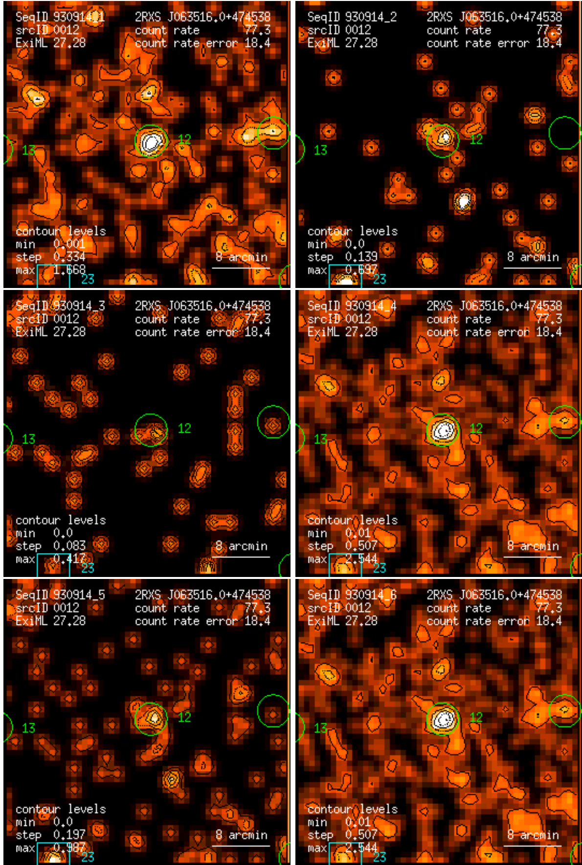
Figure 12: RASS 930914: detection 0012: band rate images, Gaussian filter: (1) PSPC channels 11 – 41, (2) 52 – 90, (3) 91 – 201, (4) 11 – 235, (5) 52 – 201, (6) 11 – 201. Broad band rates in counts/ks. Band rate contour levels in counts/ks/arcmin 2 .
