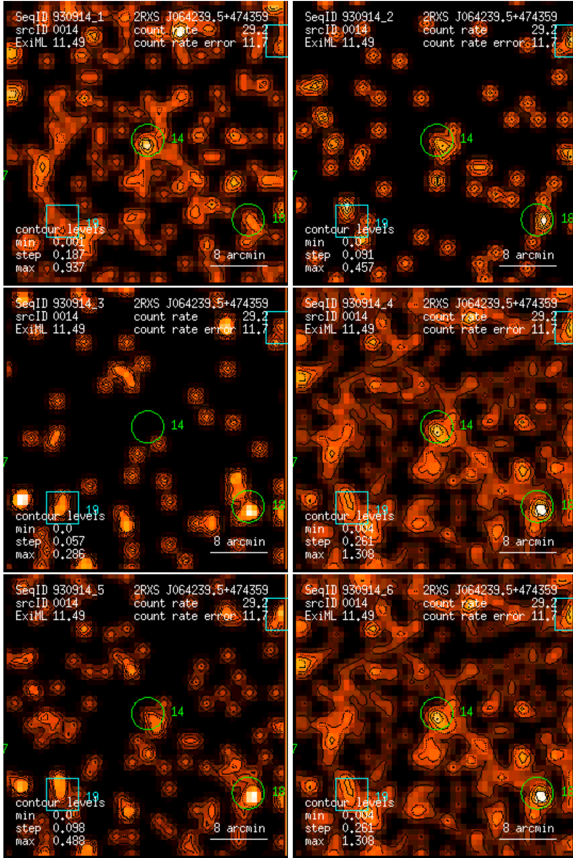
Figure 14: RASS 930914: detection 0014: band rate images, Gaussian filter: (1) PSPC channels 11 – 41, (2) 52 – 90, (3) 91 – 201, (4) 11 – 235, (5) 52 – 201, (6) 11 – 201. Broad band rates in counts/ks. Band rate contour levels in counts/ks/arcmin 2 .
