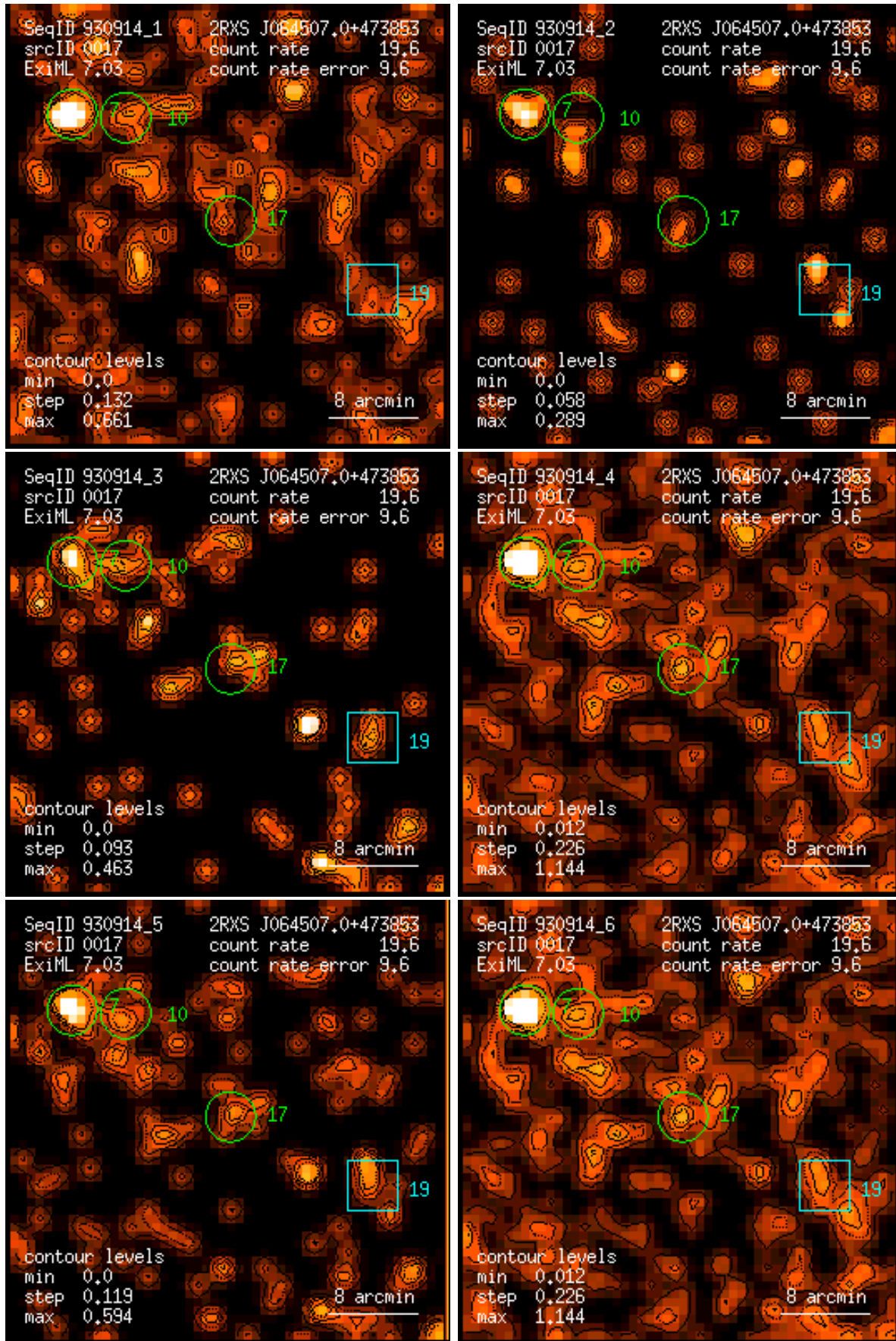
Figure 17: RASS 930914: detection 0017: band rate images, Gaussian filter: (1) PSPC channels 11 – 41, (2) 52 – 90, (3) 91 – 201, (4) 11 – 235, (5) 52 – 201, (6) 11 – 201. Broad band rates in counts/ks. Band rate contour levels in counts/ks/arcmin 2 .
