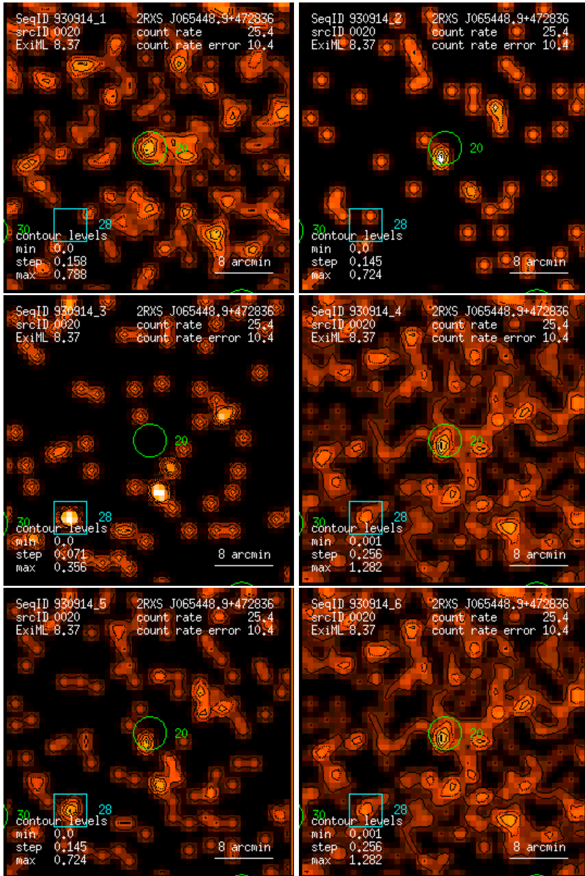
Figure 20: RASS 930914: detection 0020: band rate images, Gaussian filter: (1) PSPC channels 11 – 41, (2) 52 – 90, (3) 91 – 201, (4) 11 – 235, (5) 52 – 201, (6) 11 – 201. Broad band rates in counts/ks. Band rate contour levels in counts/ks/arcmin 2 .
