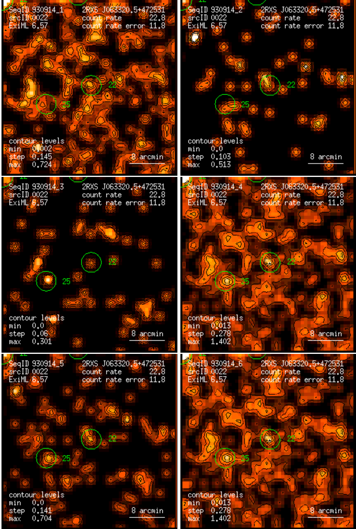
Figure 22: RASS 930914: detection 0022: band rate images, Gaussian filter: (1) PSPC channels 11 – 41, (2) 52 – 90, (3) 91 – 201, (4) 11 – 235, (5) 52 – 201, (6) 11 – 201. Broad band rates in counts/ks. Band rate contour levels in counts/ks/arcmin 2 .
