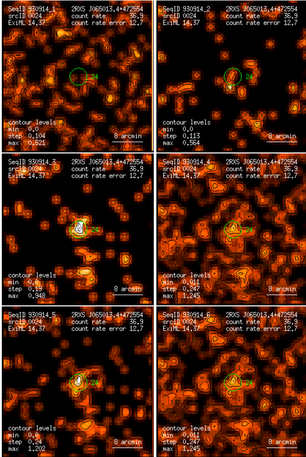
Figure 24: RASS 930914: detection 0024: band rate images, Gaussian filter: (1) PSPC channels 11 – 41, (2) 52 – 90, (3) 91 – 201, (4) 11 – 235, (5) 52 – 201, (6) 11 – 201. Broad band rates in counts/ks. Band rate contour levels in counts/ks/arcmin 2 .
