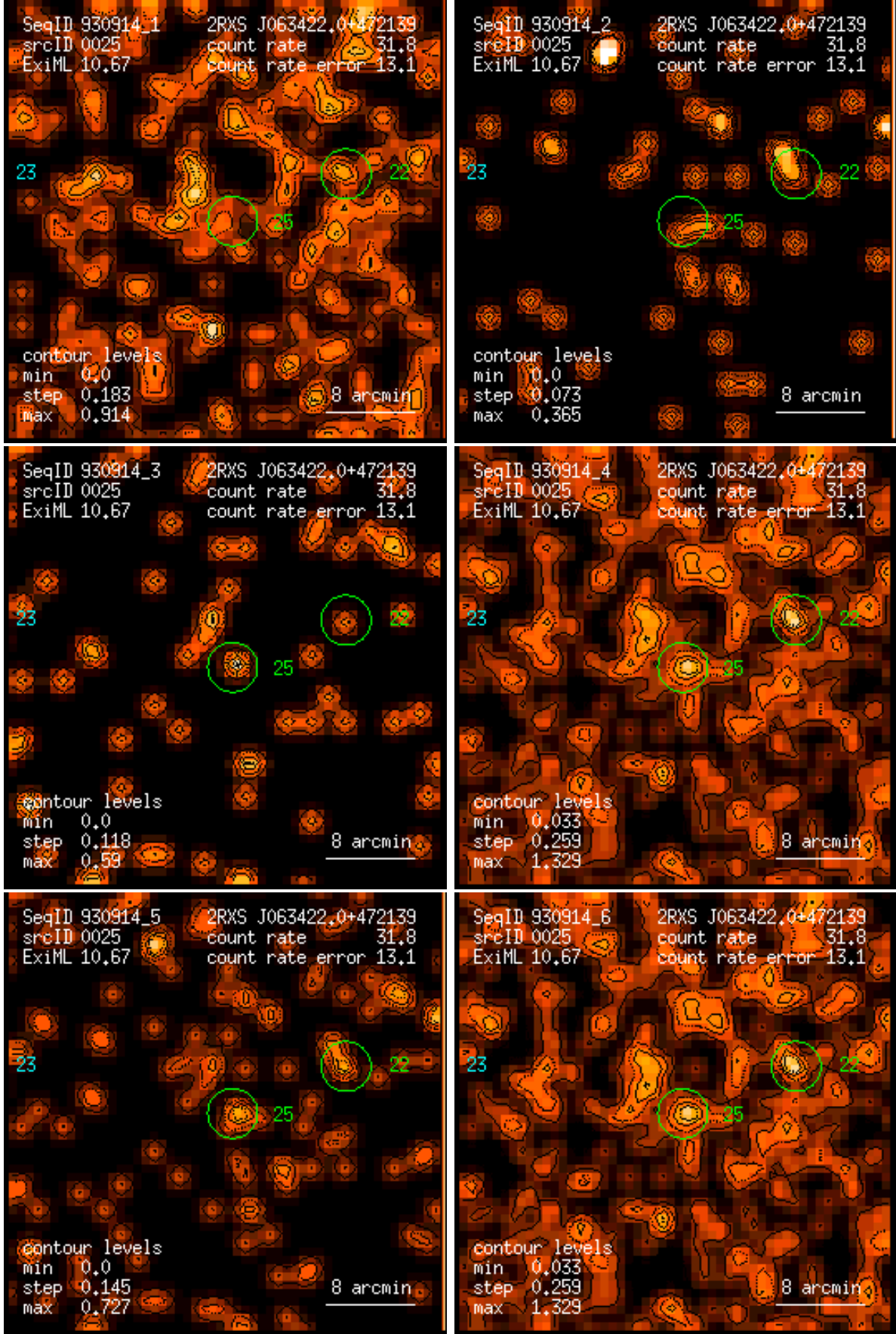
Figure 25: RASS 930914: detection 0025: band rate images, Gaussian filter: (1) PSPC channels 11 – 41, (2) 52 – 90, (3) 91 – 201, (4) 11 – 235, (5) 52 – 201, (6) 11 – 201. Broad band rates in counts/ks. Band rate contour levels in counts/ks/arcmin 2 .
