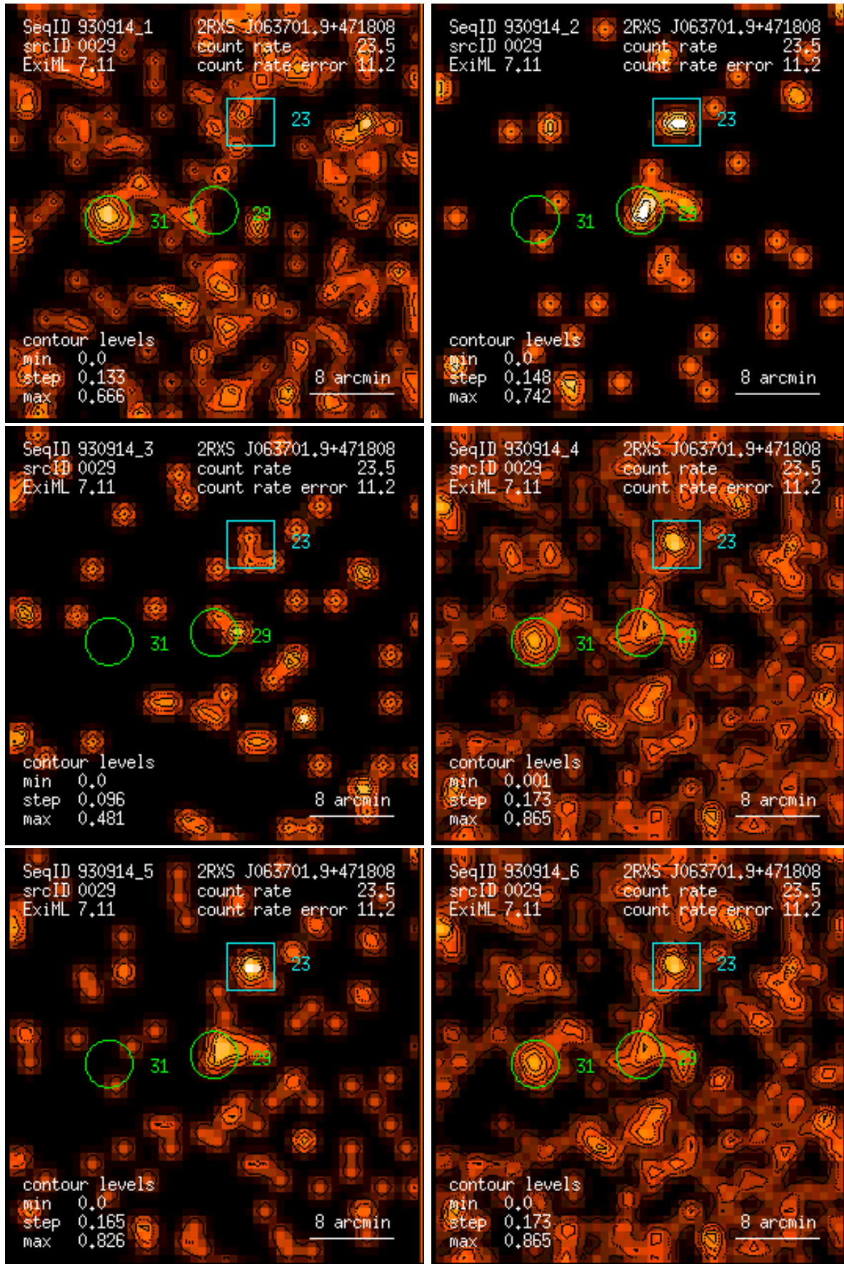
Figure 29: RASS 930914: detection 0029: band rate images, Gaussian filter: (1) PSPC channels 11 – 41, (2) 52 – 90, (3) 91 – 201, (4) 11 – 235, (5) 52 – 201, (6) 11 – 201. Broad band rates in counts/ks. Band rate contour levels in counts/ks/arcmin 2 .
