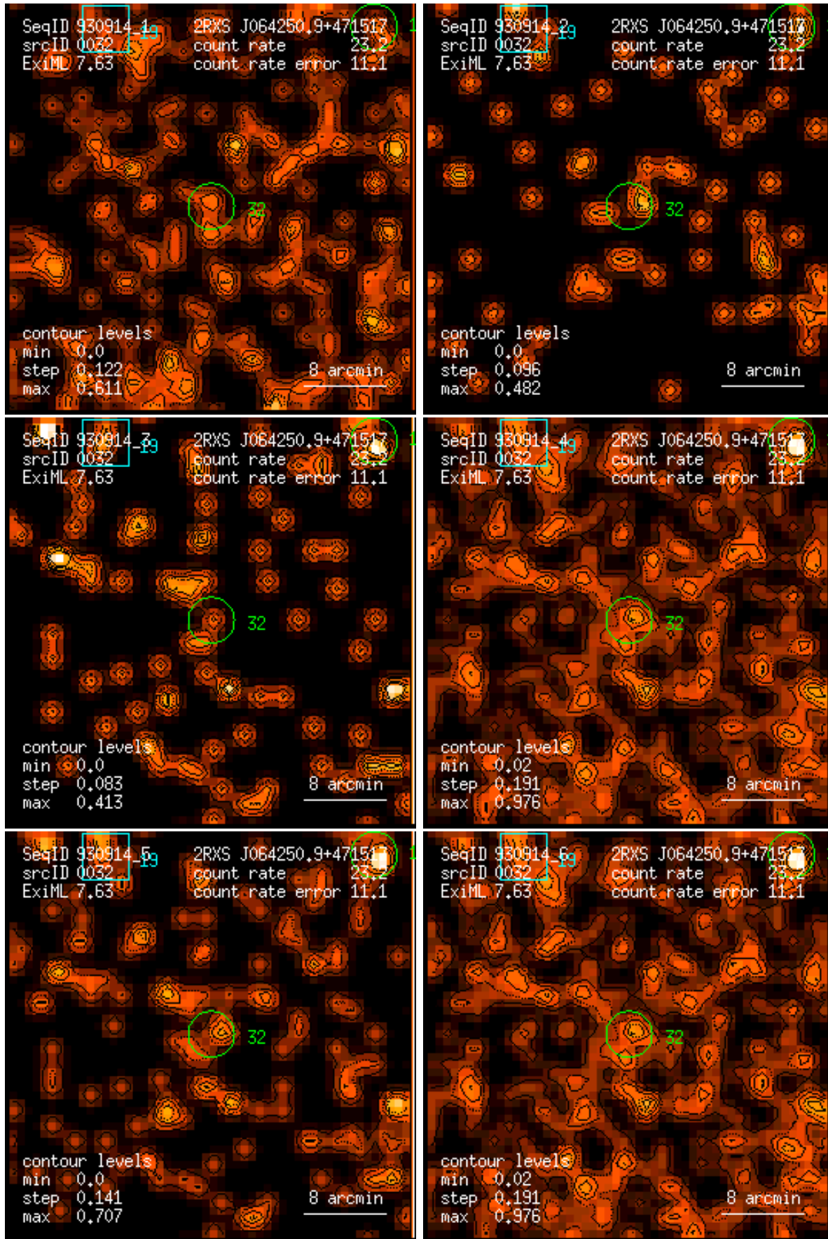
Figure 32: RASS 930914: detection 0032: band rate images, Gaussian filter: (1) PSPC channels 11 – 41, (2) 52 – 90, (3) 91 – 201, (4) 11 – 235, (5) 52 – 201, (6) 11 – 201. Broad band rates in counts/ks. Band rate contour levels in counts/ks/arcmin 2 .
