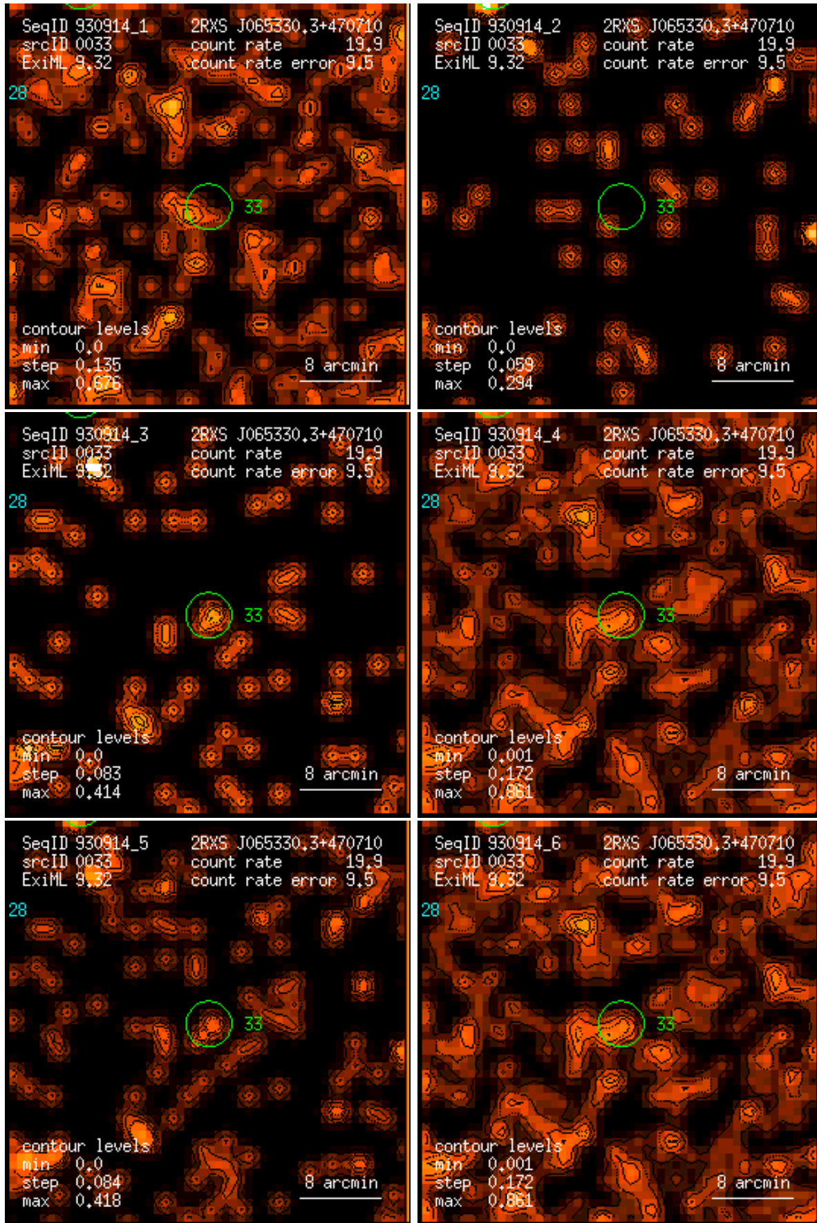
Figure 33: RASS 930914: detection 0033: band rate images, Gaussian filter: (1) PSPC channels 11 – 41, (2) 52 – 90, (3) 91 – 201, (4) 11 – 235, (5) 52 – 201, (6) 11 – 201. Broad band rates in counts/ks. Band rate contour levels in counts/ks/arcmin 2 .
