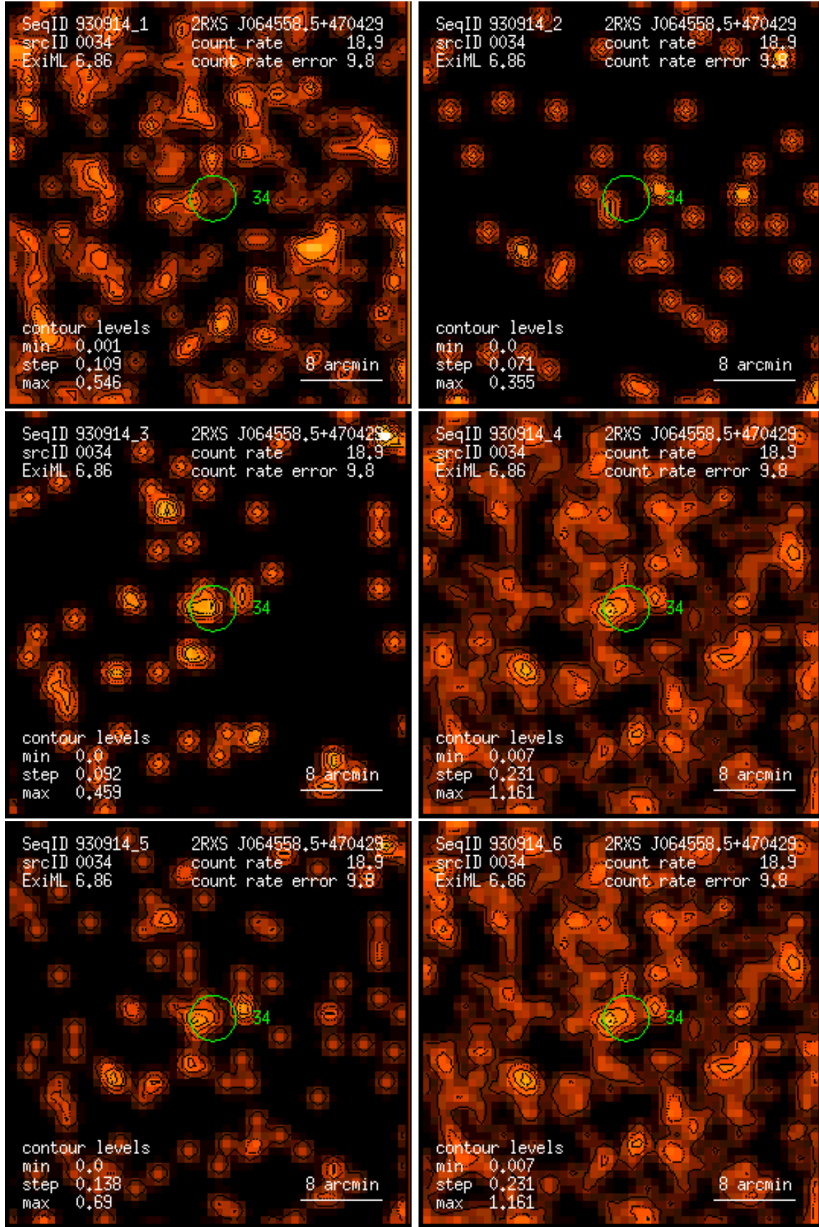
Figure 34: RASS 930914: detection 0034: band rate images, Gaussian filter: (1) PSPC channels 11 – 41, (2) 52 – 90, (3) 91 – 201, (4) 11 – 235, (5) 52 – 201, (6) 11 – 201. Broad band rates in counts/ks. Band rate contour levels in counts/ks/arcmin 2 .
