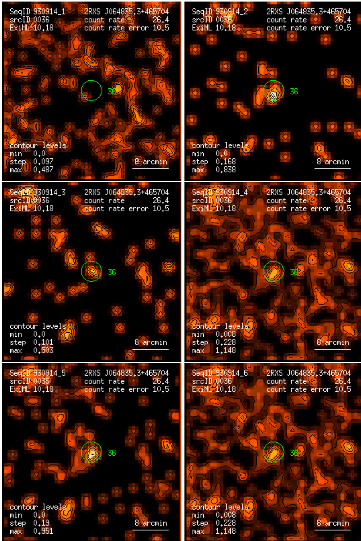
Figure 36: RASS 930914: detection 0036: band rate images, Gaussian filter: (1) PSPC channels 11 – 41, (2) 52 – 90, (3) 91 – 201, (4) 11 – 235, (5) 52 – 201, (6) 11 – 201. Broad band rates in counts/ks. Band rate contour levels in counts/ks/arcmin 2 .
