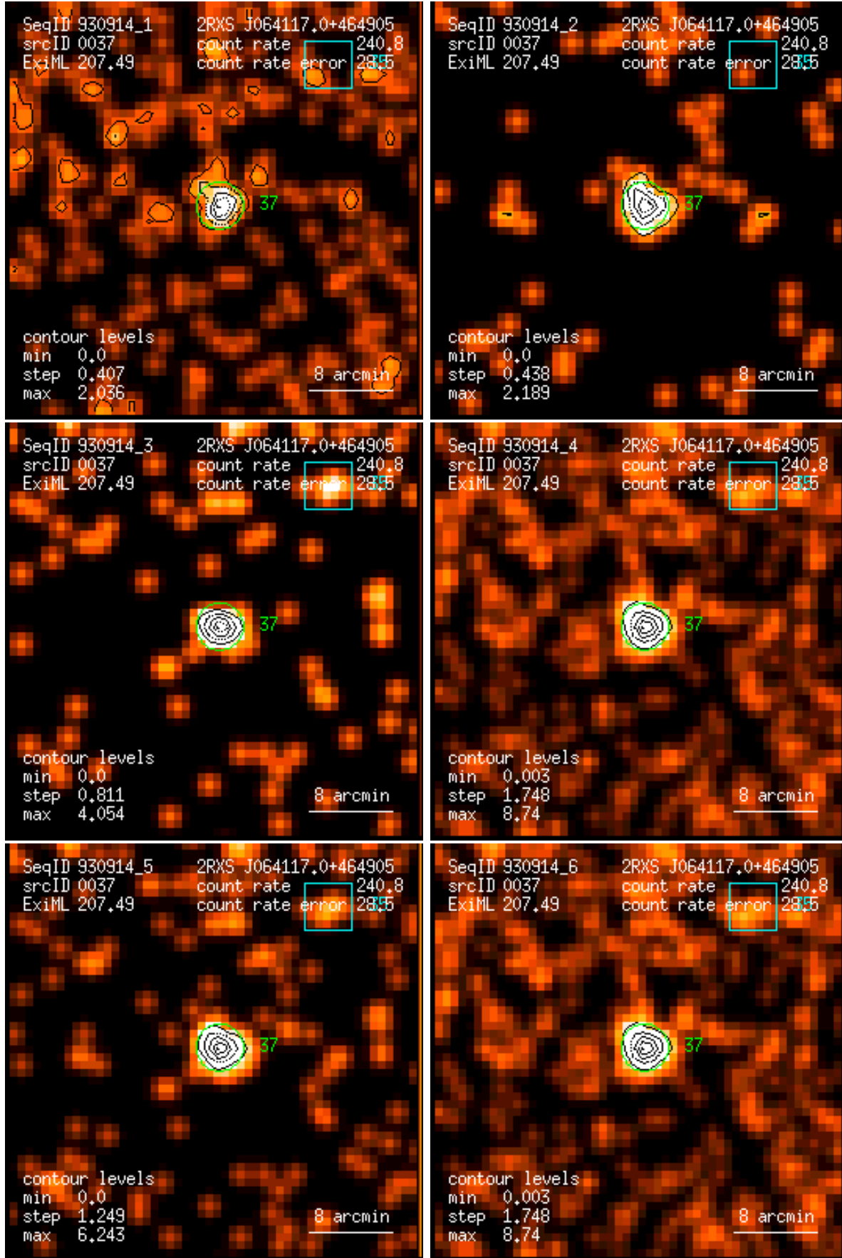
Figure 37: RASS 930914: detection 0037: band rate images, Gaussian filter: (1) PSPC channels 11 – 41, (2) 52 – 90, (3) 91 – 201, (4) 11 – 235, (5) 52 – 201, (6) 11 – 201. Broad band rates in counts/ks. Band rate contour levels in counts/ks/arcmin 2 .
