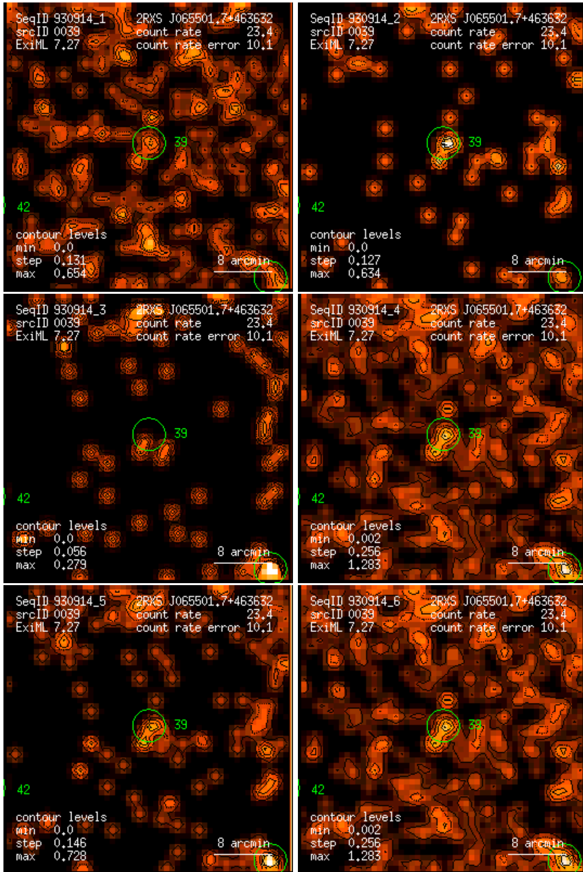
Figure 39: RASS 930914: detection 0039: band rate images, Gaussian filter: (1) PSPC channels 11 – 41, (2) 52 – 90, (3) 91 – 201, (4) 11 – 235, (5) 52 – 201, (6) 11 – 201. Broad band rates in counts/ks. Band rate contour levels in counts/ks/arcmin 2 .
