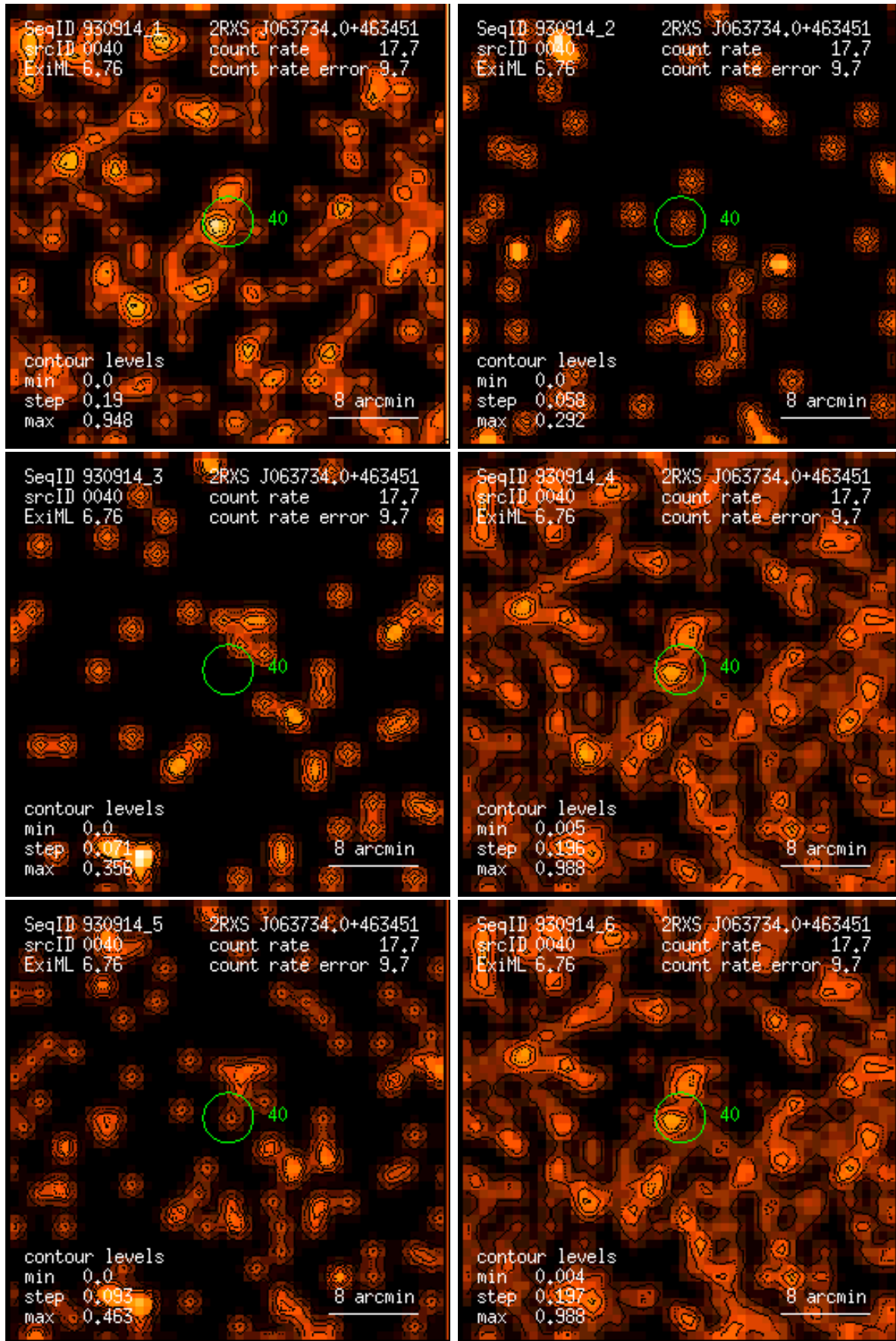
Figure 40: RASS 930914: detection 0040: band rate images, Gaussian filter: (1) PSPC channels 11 – 41, (2) 52 – 90, (3) 91 – 201, (4) 11 – 235, (5) 52 – 201, (6) 11 – 201. Broad band rates in counts/ks. Band rate contour levels in counts/ks/arcmin 2 .
