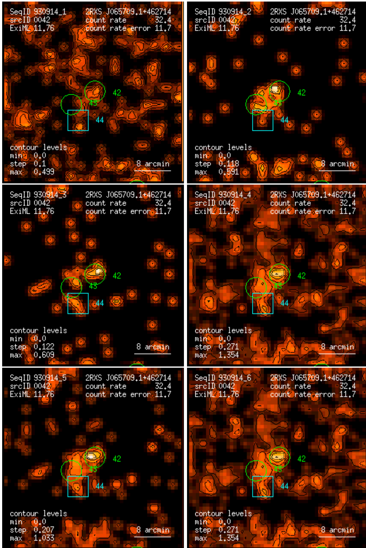
Figure 42: RASS 930914: detection 0042: band rate images, Gaussian filter: (1) PSPC channels 11 – 41, (2) 52 – 90, (3) 91 – 201, (4) 11 – 235, (5) 52 – 201, (6) 11 – 201. Broad band rates in counts/ks. Band rate contour levels in counts/ks/arcmin 2 .
