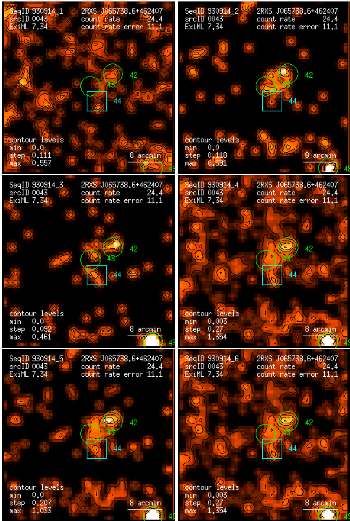
Figure 43: RASS 930914: detection 0043: band rate images, Gaussian filter: (1) PSPC channels 11 – 41, (2) 52 – 90, (3) 91 – 201, (4) 11 – 235, (5) 52 – 201, (6) 11 – 201. Broad band rates in counts/ks. Band rate contour levels in counts/ks/arcmin 2 .
