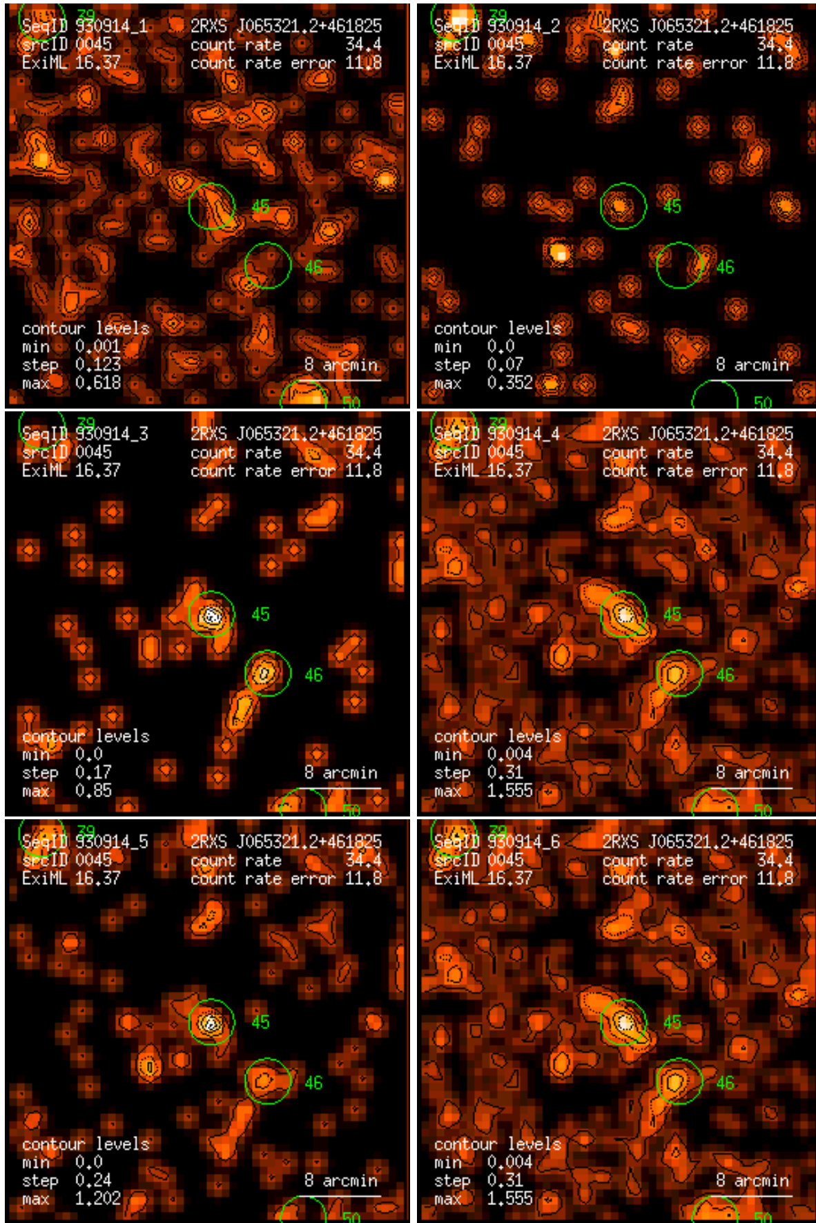
Figure 45: RASS 930914: detection 0045: band rate images, Gaussian filter: (1) PSPC channels 11 – 41, (2) 52 – 90, (3) 91 – 201, (4) 11 – 235, (5) 52 – 201, (6) 11 – 201. Broad band rates in counts/ks. Band rate contour levels in counts/ks/arcmin 2 .
