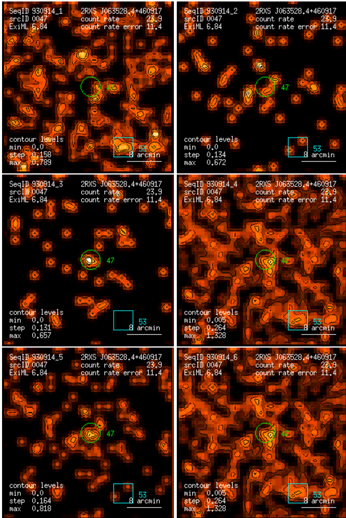
Figure 47: RASS 930914: detection 0047: band rate images, Gaussian filter: (1) PSPC channels 11 – 41, (2) 52 – 90, (3) 91 – 201, (4) 11 – 235, (5) 52 – 201, (6) 11 – 201. Broad band rates in counts/ks. Band rate contour levels in counts/ks/arcmin 2 .
