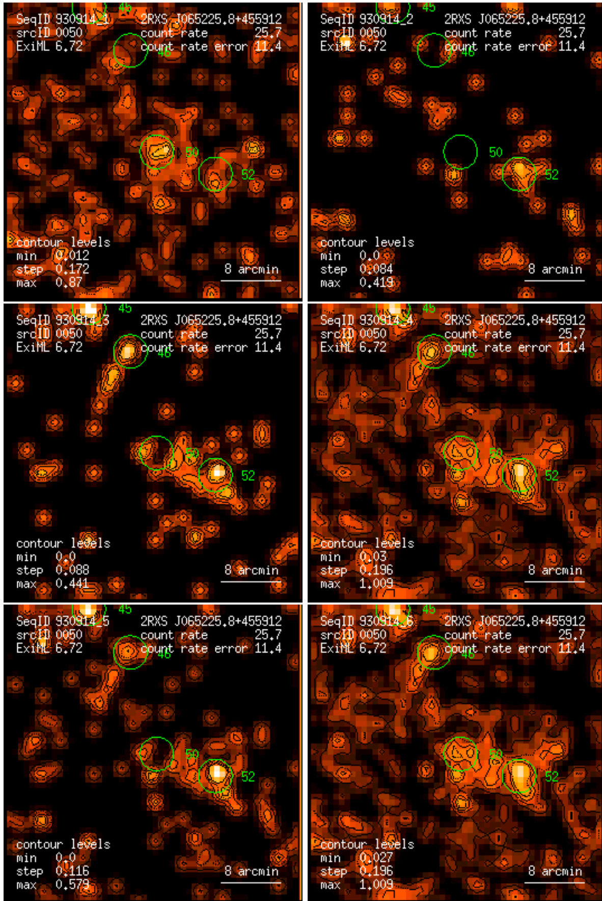
Figure 50: RASS 930914: detection 0050: band rate images, Gaussian filter: (1) PSPC channels 11 – 41, (2) 52 – 90, (3) 91 – 201, (4) 11 – 235, (5) 52 – 201, (6) 11 – 201. Broad band rates in counts/ks. Band rate contour levels in counts/ks/arcmin 2 .
