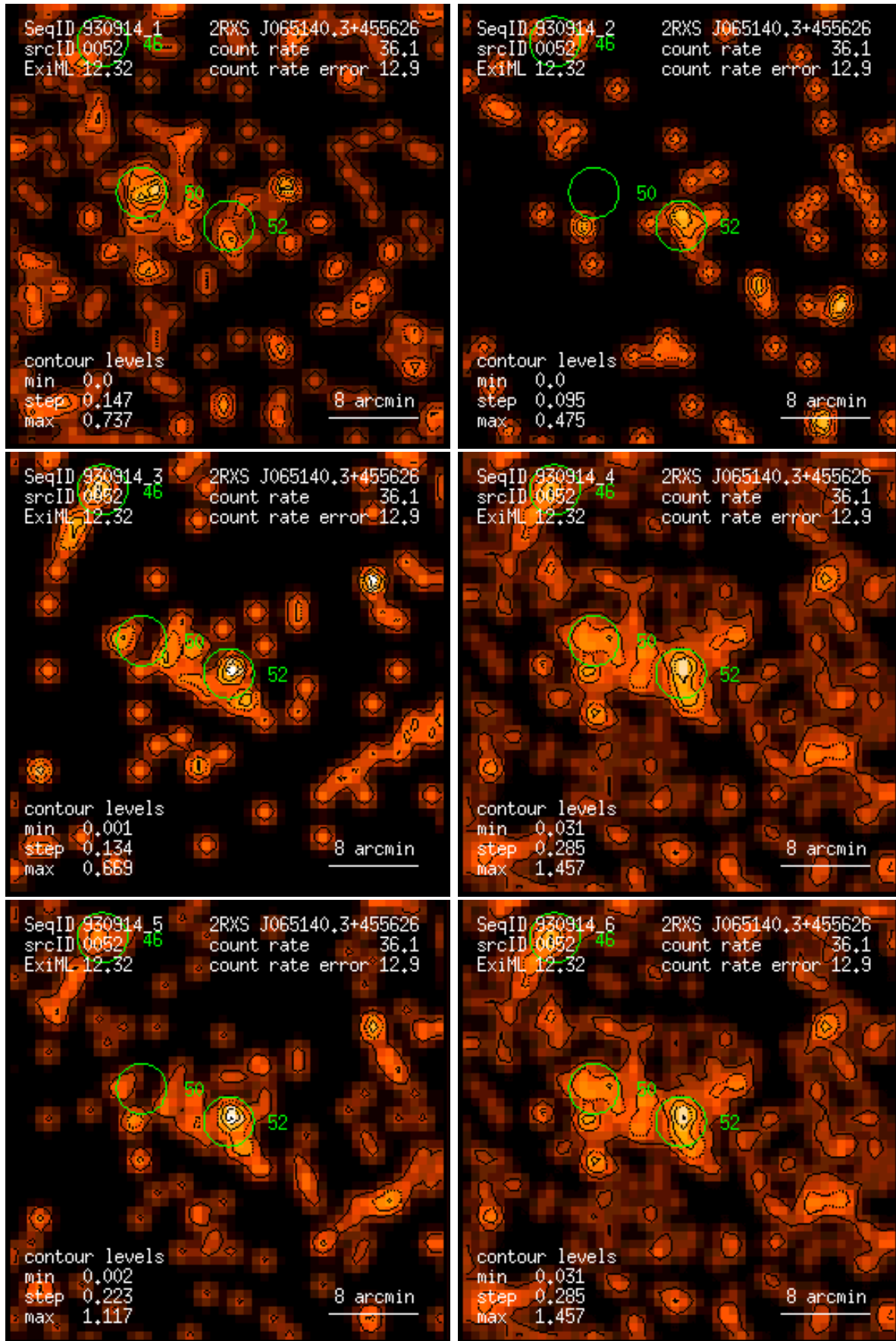
Figure 52: RASS 930914: detection 0052: band rate images, Gaussian filter: (1) PSPC channels 11 – 41, (2) 52 – 90, (3) 91 – 201, (4) 11 – 235, (5) 52 – 201, (6) 11 – 201. Broad band rates in counts/ks. Band rate contour levels in counts/ks/arcmin 2 .
