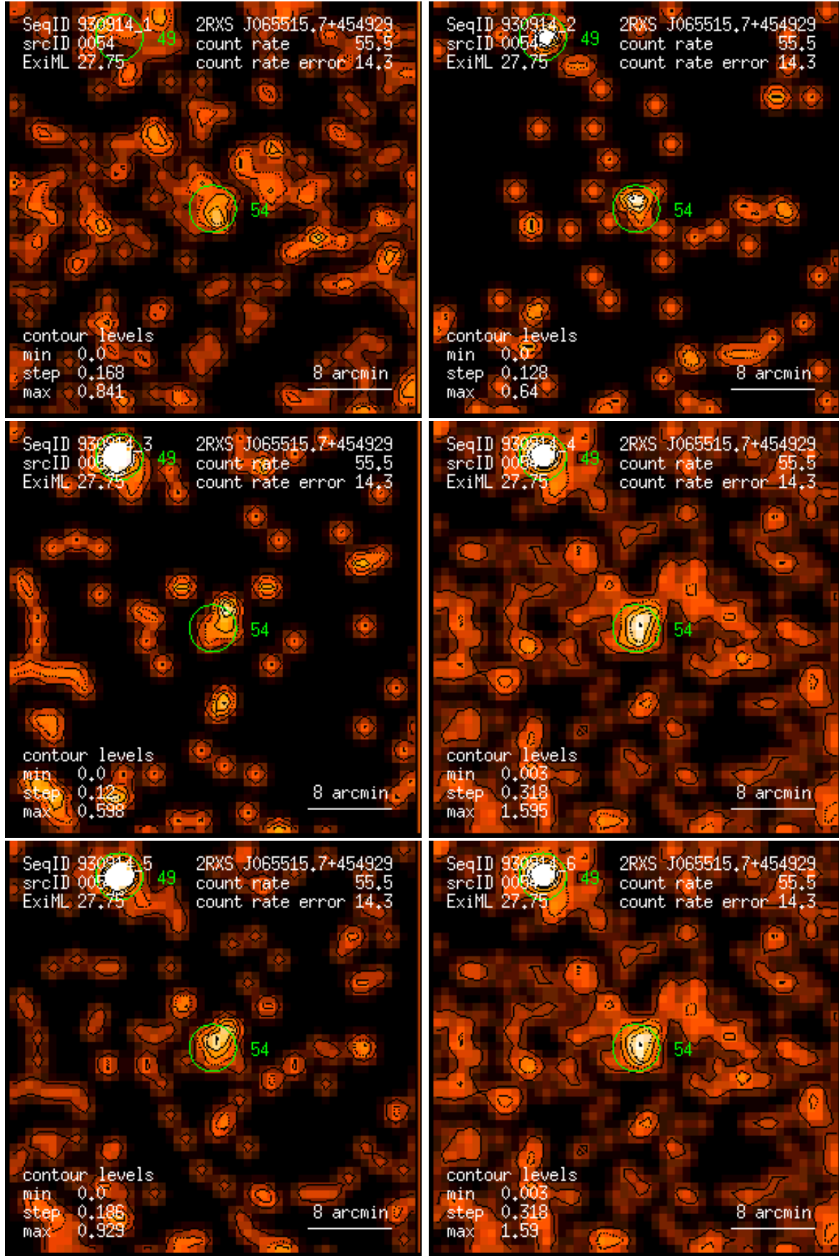
Figure 54: RASS 930914: detection 0054: band rate images, Gaussian filter: (1) PSPC channels 11 – 41, (2) 52 – 90, (3) 91 – 201, (4) 11 – 235, (5) 52 – 201, (6) 11 – 201. Broad band rates in counts/ks. Band rate contour levels in counts/ks/arcmin 2 .
