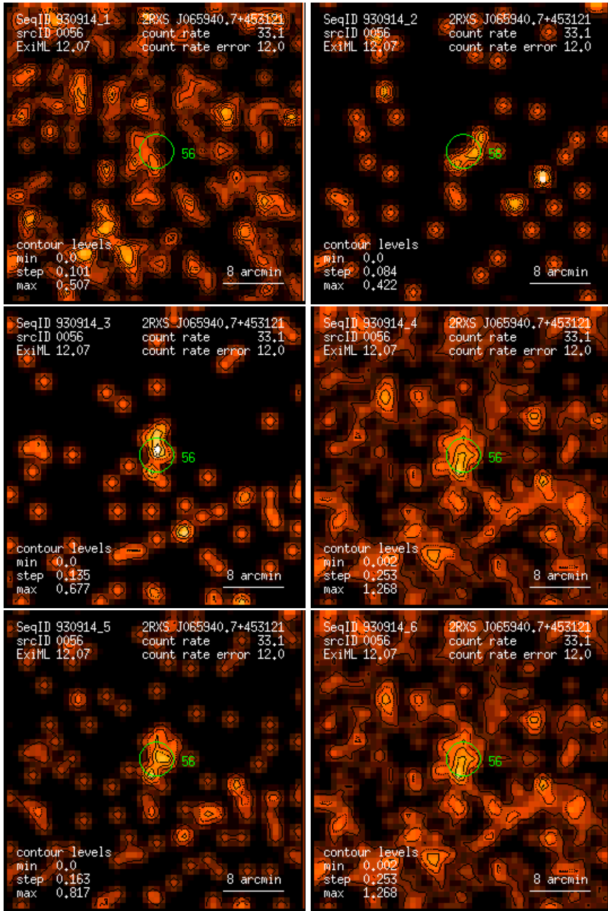
Figure 56: RASS 930914: detection 0056: band rate images, Gaussian filter: (1) PSPC channels 11 – 41, (2) 52 – 90, (3) 91 – 201, (4) 11 – 235, (5) 52 – 201, (6) 11 – 201. Broad band rates in counts/ks. Band rate contour levels in counts/ks/arcmin 2 .
