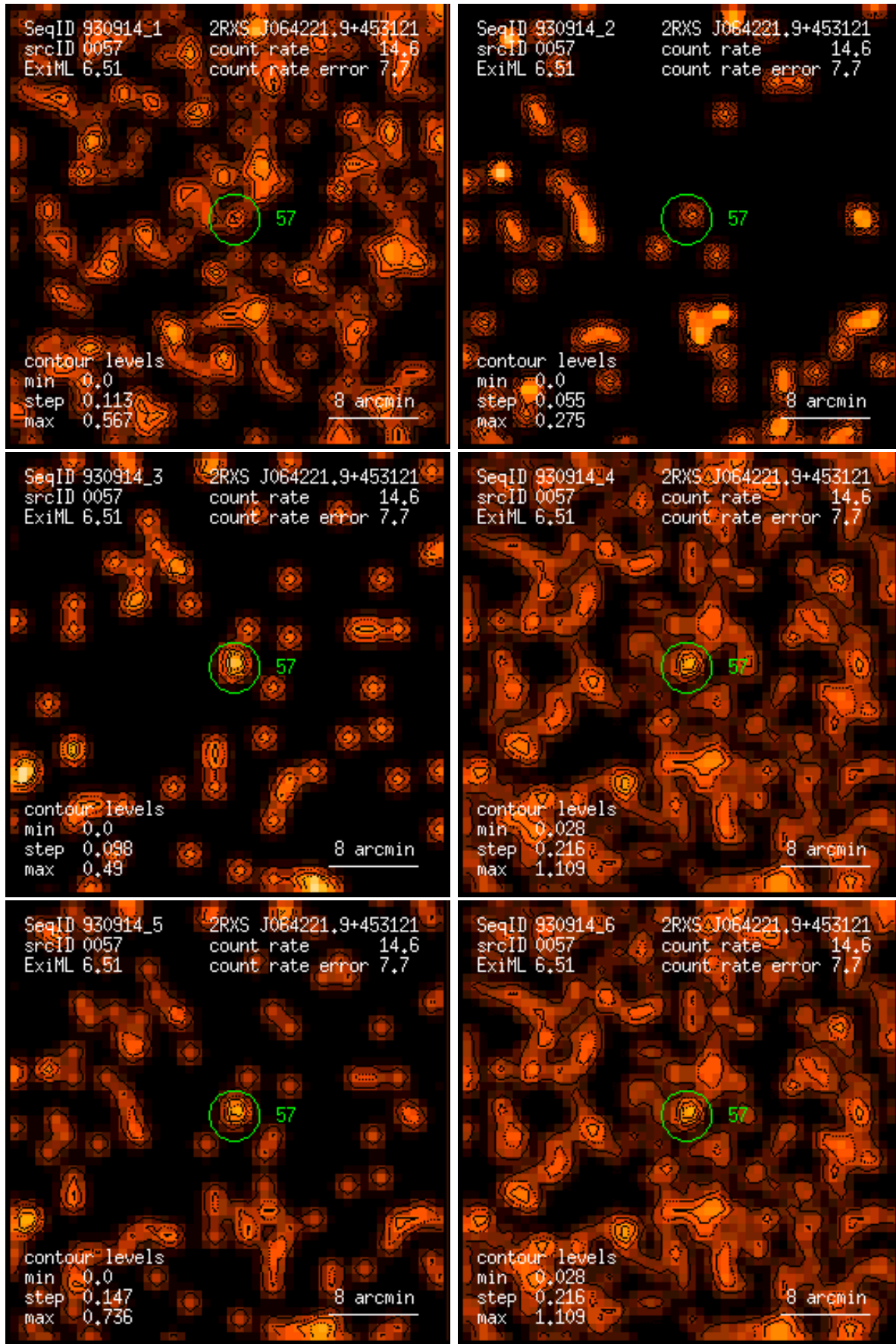
Figure 57: RASS 930914: detection 0057: band rate images, Gaussian filter: (1) PSPC channels 11 – 41, (2) 52 – 90, (3) 91 – 201, (4) 11 – 235, (5) 52 – 201, (6) 11 – 201. Broad band rates in counts/ks. Band rate contour levels in counts/ks/arcmin 2 .
