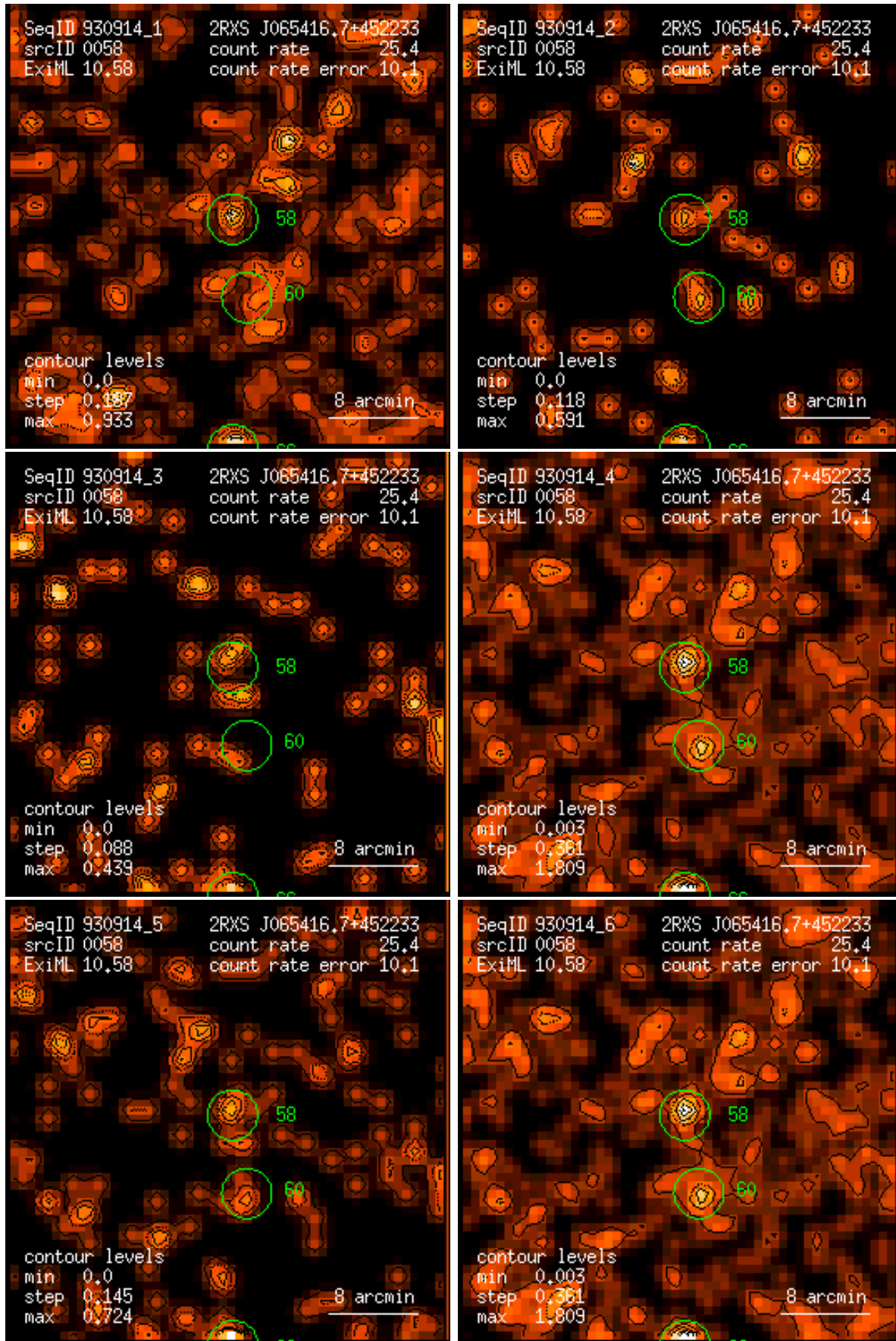
Figure 58: RASS 930914: detection 0058: band rate images, Gaussian filter: (1) PSPC channels 11 – 41, (2) 52 – 90, (3) 91 – 201, (4) 11 – 235, (5) 52 – 201, (6) 11 – 201. Broad band rates in counts/ks. Band rate contour levels in counts/ks/arcmin 2 .
