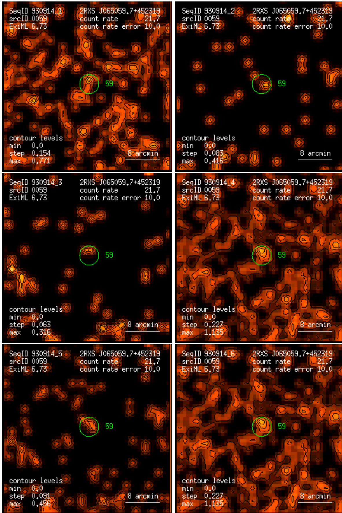
Figure 59: RASS 930914: detection 0059: band rate images, Gaussian filter: (1) PSPC channels 11 – 41, (2) 52 – 90, (3) 91 – 201, (4) 11 – 235, (5) 52 – 201, (6) 11 – 201. Broad band rates in counts/ks. Band rate contour levels in counts/ks/arcmin 2 .
