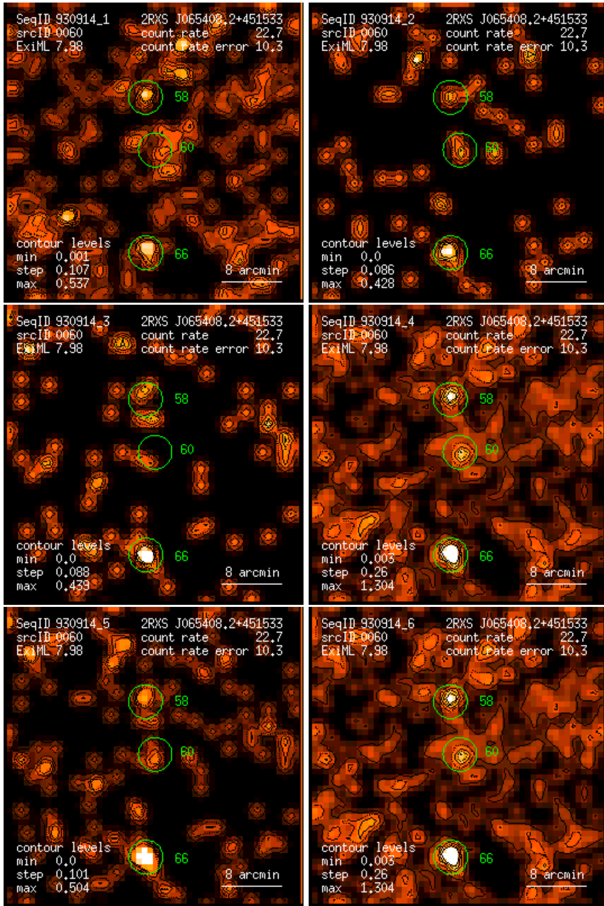
Figure 60: RASS 930914: detection 0060: band rate images, Gaussian filter: (1) PSPC channels 11 – 41, (2) 52 – 90, (3) 91 – 201, (4) 11 – 235, (5) 52 – 201, (6) 11 – 201. Broad band rates in counts/ks. Band rate contour levels in counts/ks/arcmin 2 .
