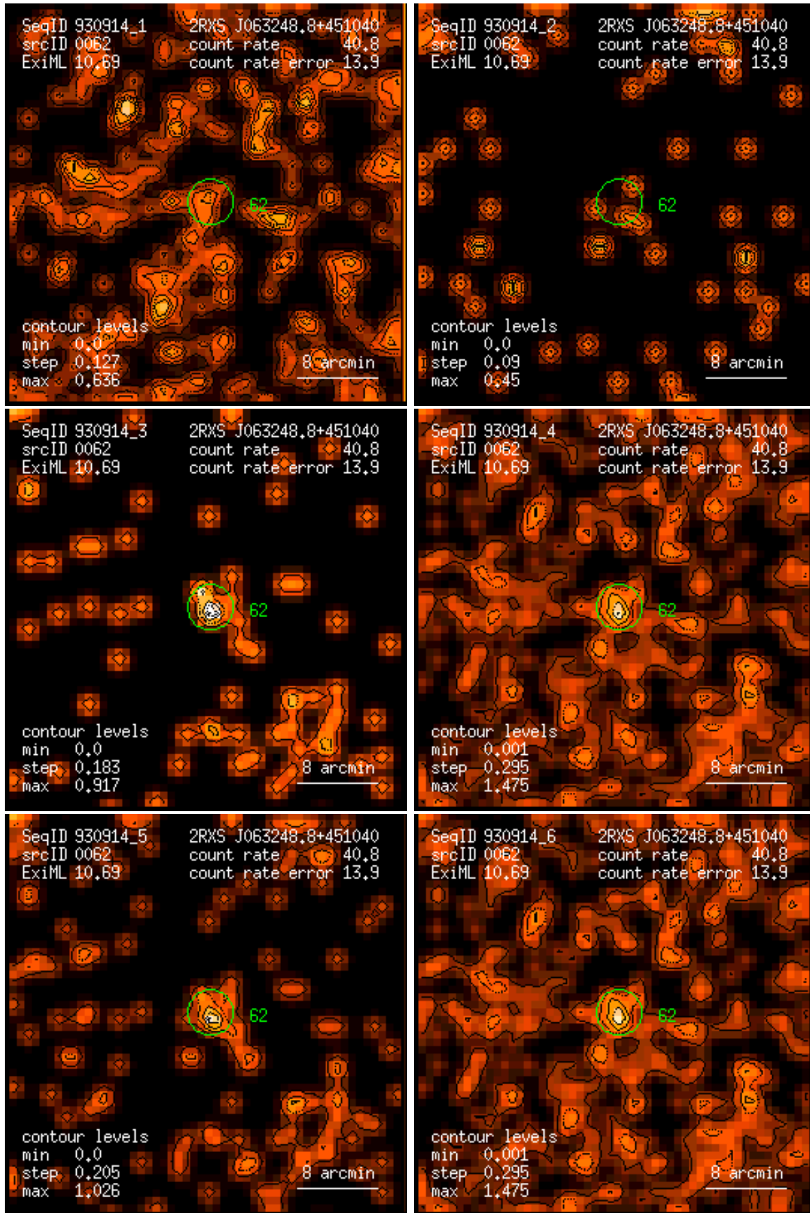
Figure 62: RASS 930914: detection 0062: band rate images, Gaussian filter: (1) PSPC channels 11 – 41, (2) 52 – 90, (3) 91 – 201, (4) 11 – 235, (5) 52 – 201, (6) 11 – 201. Broad band rates in counts/ks. Band rate contour levels in counts/ks/arcmin 2 .
