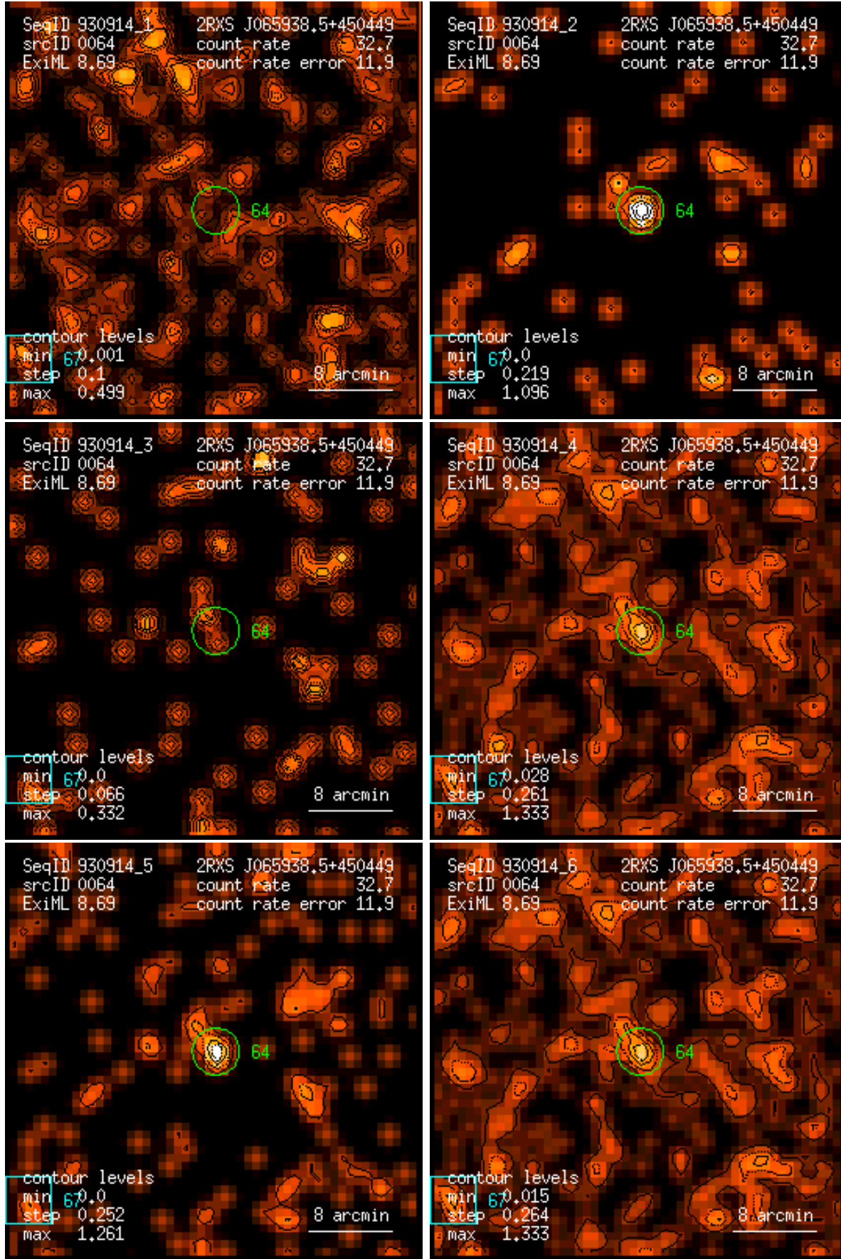
Figure 64: RASS 930914: detection 0064: band rate images, Gaussian filter: (1) PSPC channels 11 – 41, (2) 52 – 90, (3) 91 – 201, (4) 11 – 235, (5) 52 – 201, (6) 11 – 201. Broad band rates in counts/ks. Band rate contour levels in counts/ks/arcmin 2 .
