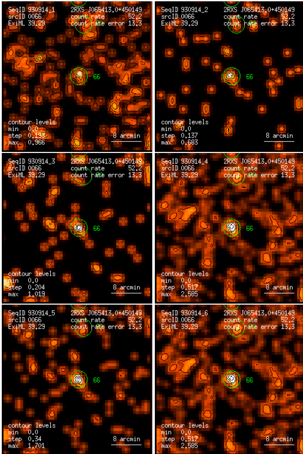
Figure 66: RASS 930914: detection 0066: band rate images, Gaussian filter: (1) PSPC channels 11 – 41, (2) 52 – 90, (3) 91 – 201, (4) 11 – 235, (5) 52 – 201, (6) 11 – 201. Broad band rates in counts/ks. Band rate contour levels in counts/ks/arcmin 2 .
