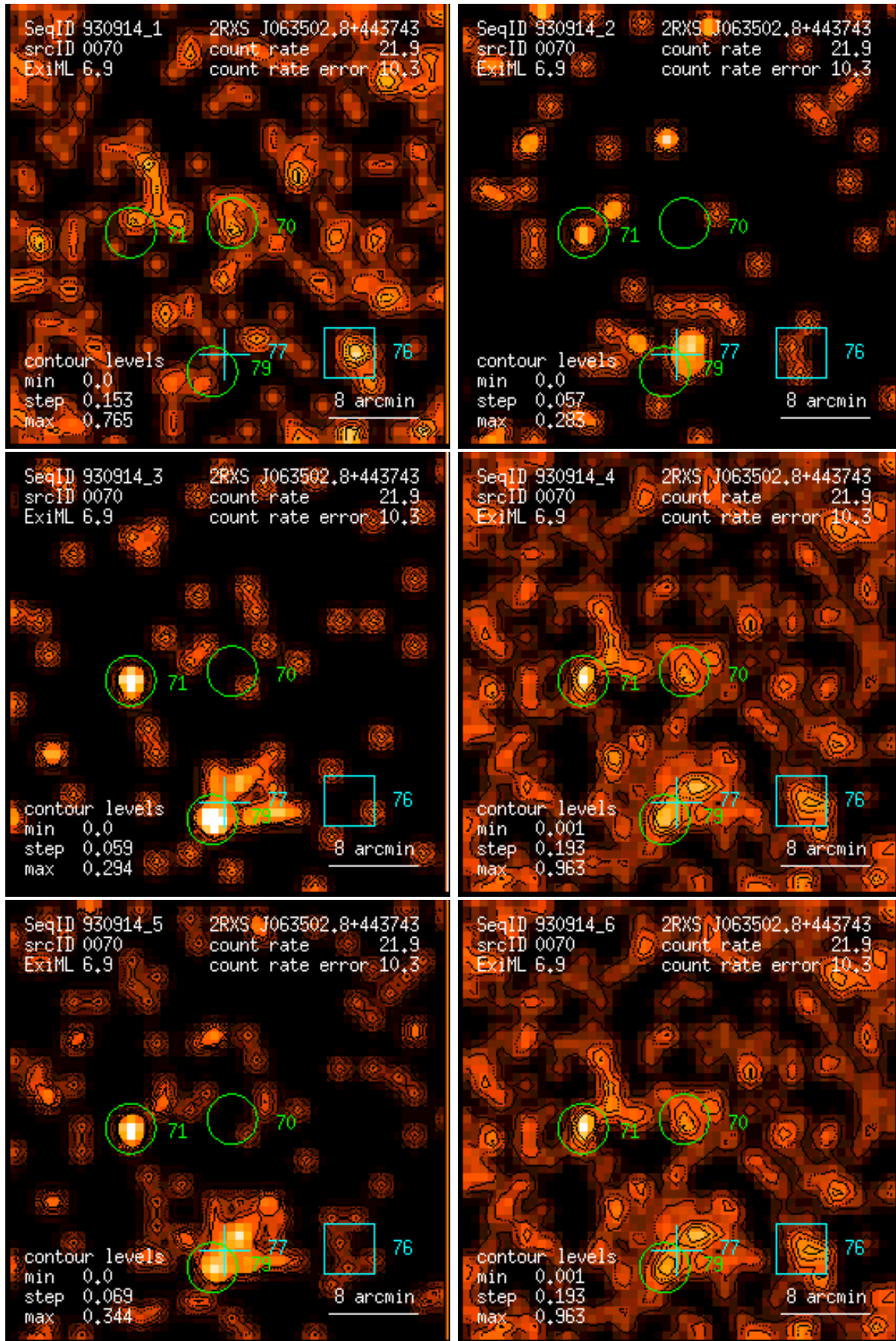
Figure 70: RASS 930914: detection 0070: band rate images, Gaussian filter: (1) PSPC channels 11 – 41, (2) 52 – 90, (3) 91 – 201, (4) 11 – 235, (5) 52 – 201, (6) 11 – 201. Broad band rates in counts/ks. Band rate contour levels in counts/ks/arcmin 2 .
