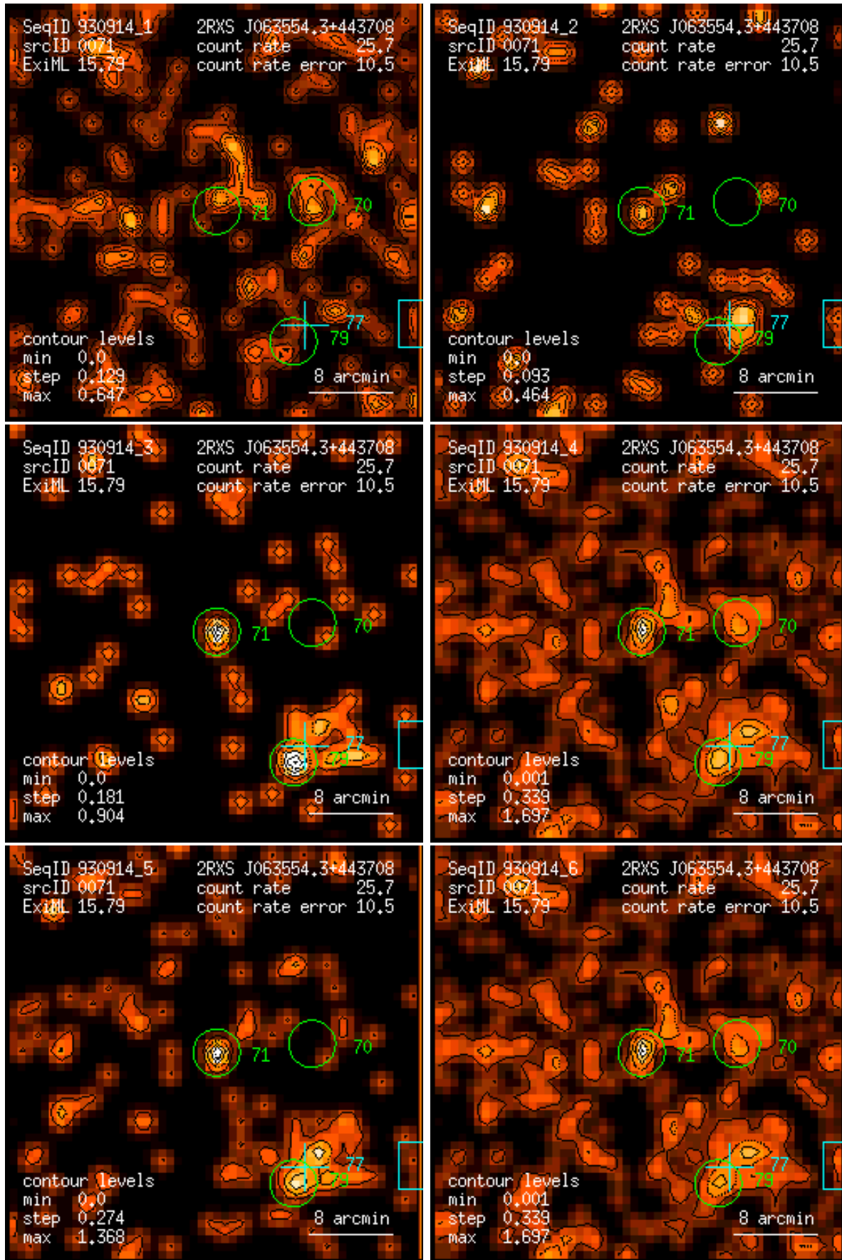
Figure 71: RASS 930914: detection 0071: band rate images, Gaussian filter: (1) PSPC channels 11 – 41, (2) 52 – 90, (3) 91 – 201, (4) 11 – 235, (5) 52 – 201, (6) 11 – 201. Broad band rates in counts/ks. Band rate contour levels in counts/ks/arcmin 2 .
