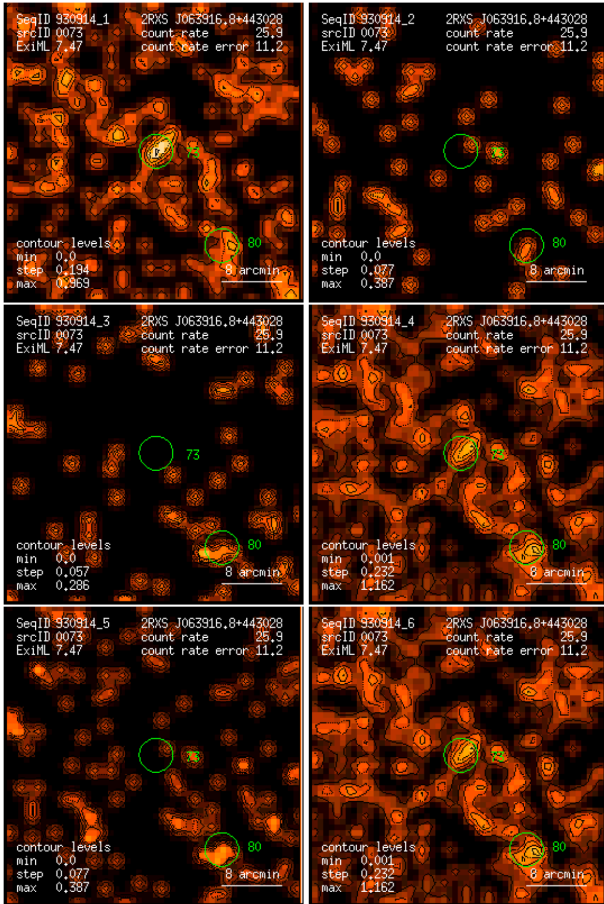
Figure 73: RASS 930914: detection 0073: band rate images, Gaussian filter: (1) PSPC channels 11 – 41, (2) 52 – 90, (3) 91 – 201, (4) 11 – 235, (5) 52 – 201, (6) 11 – 201. Broad band rates in counts/ks. Band rate contour levels in counts/ks/arcmin 2 .
