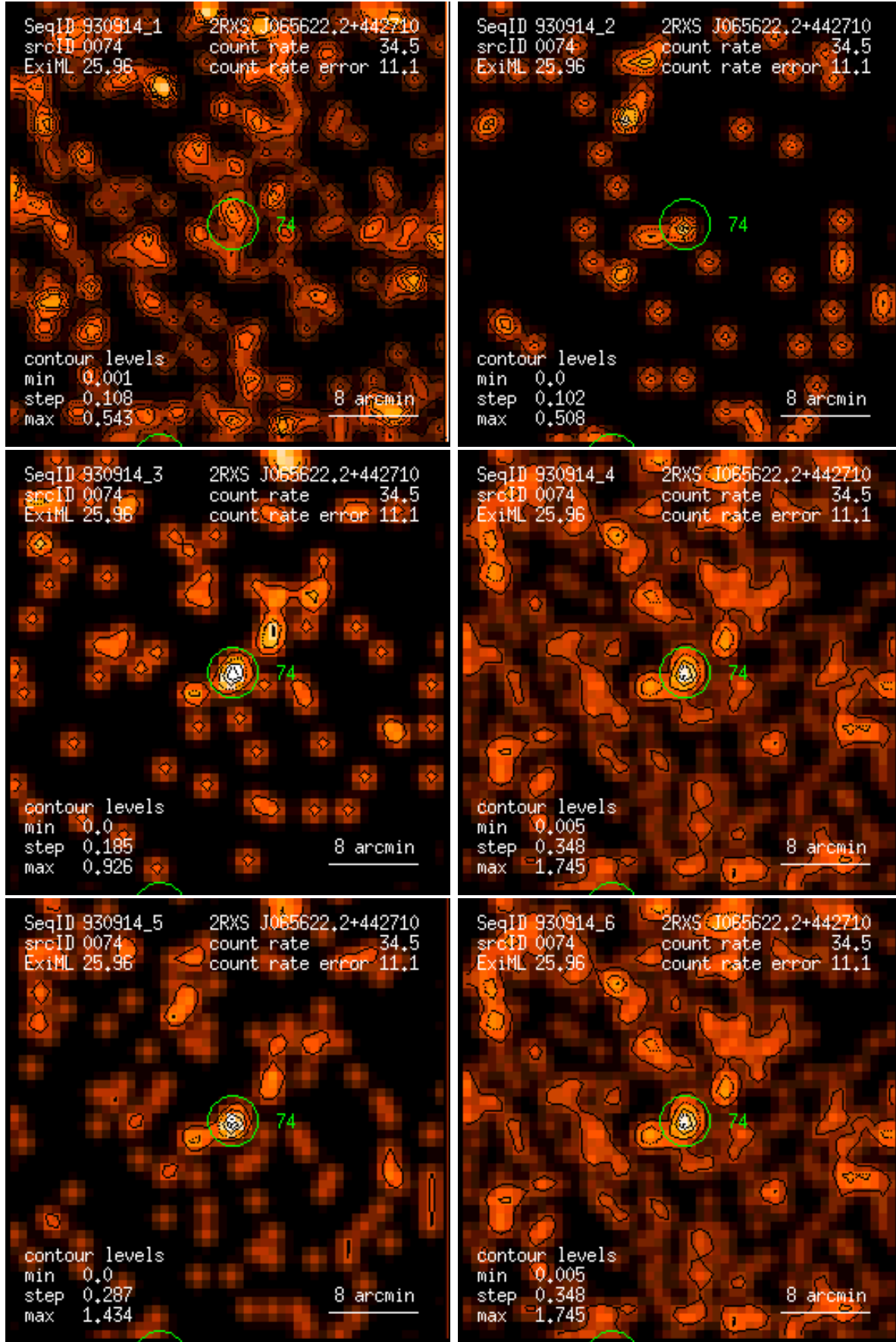
Figure 74: RASS 930914: detection 0074: band rate images, Gaussian filter: (1) PSPC channels 11 – 41, (2) 52 – 90, (3) 91 – 201, (4) 11 – 235, (5) 52 – 201, (6) 11 – 201. Broad band rates in counts/ks. Band rate contour levels in counts/ks/arcmin 2 .
