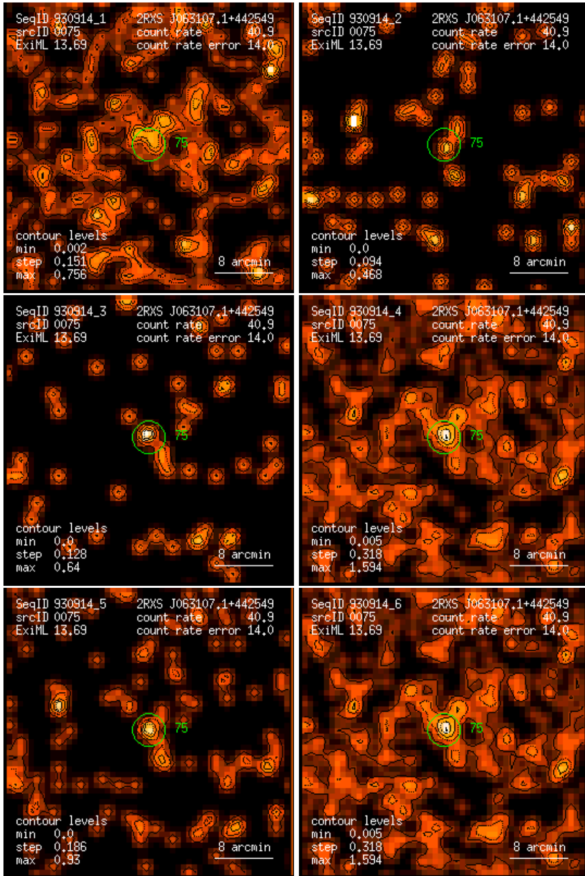
Figure 75: RASS 930914: detection 0075: band rate images, Gaussian filter: (1) PSPC channels 11 – 41, (2) 52 – 90, (3) 91 – 201, (4) 11 – 235, (5) 52 – 201, (6) 11 – 201. Broad band rates in counts/ks. Band rate contour levels in counts/ks/arcmin 2 .
