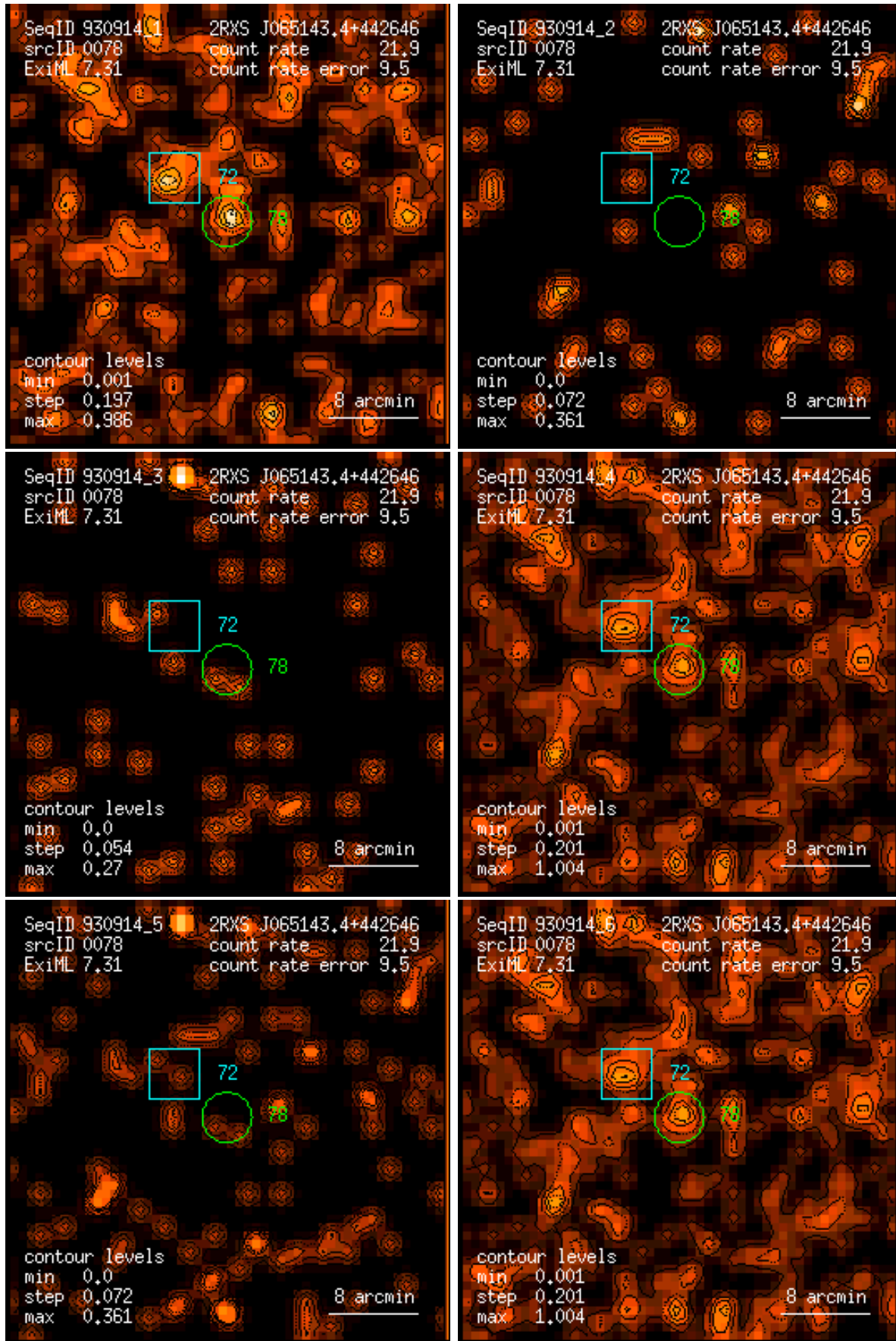
Figure 78: RASS 930914: detection 0078: band rate images, Gaussian filter: (1) PSPC channels 11 – 41, (2) 52 – 90, (3) 91 – 201, (4) 11 – 235, (5) 52 – 201, (6) 11 – 201. Broad band rates in counts/ks. Band rate contour levels in counts/ks/arcmin 2 .
