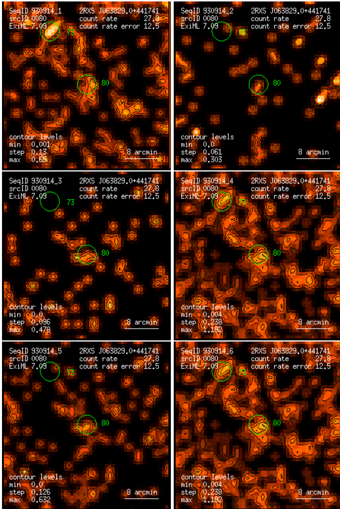
Figure 80: RASS 930914: detection 0080: band rate images, Gaussian filter: (1) PSPC channels 11 – 41, (2) 52 – 90, (3) 91 – 201, (4) 11 – 235, (5) 52 – 201, (6) 11 – 201. Broad band rates in counts/ks. Band rate contour levels in counts/ks/arcmin 2 .
