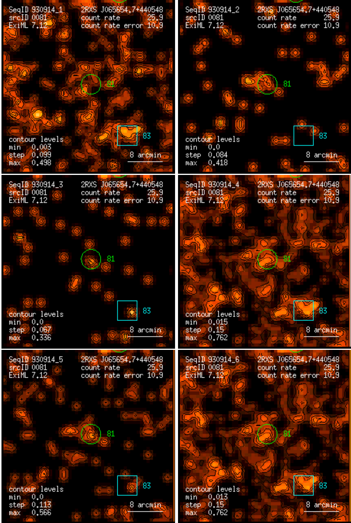
Figure 81: RASS 930914: detection 0081: band rate images, Gaussian filter: (1) PSPC channels 11 – 41, (2) 52 – 90, (3) 91 – 201, (4) 11 – 235, (5) 52 – 201, (6) 11 – 201. Broad band rates in counts/ks. Band rate contour levels in counts/ks/arcmin 2 .
