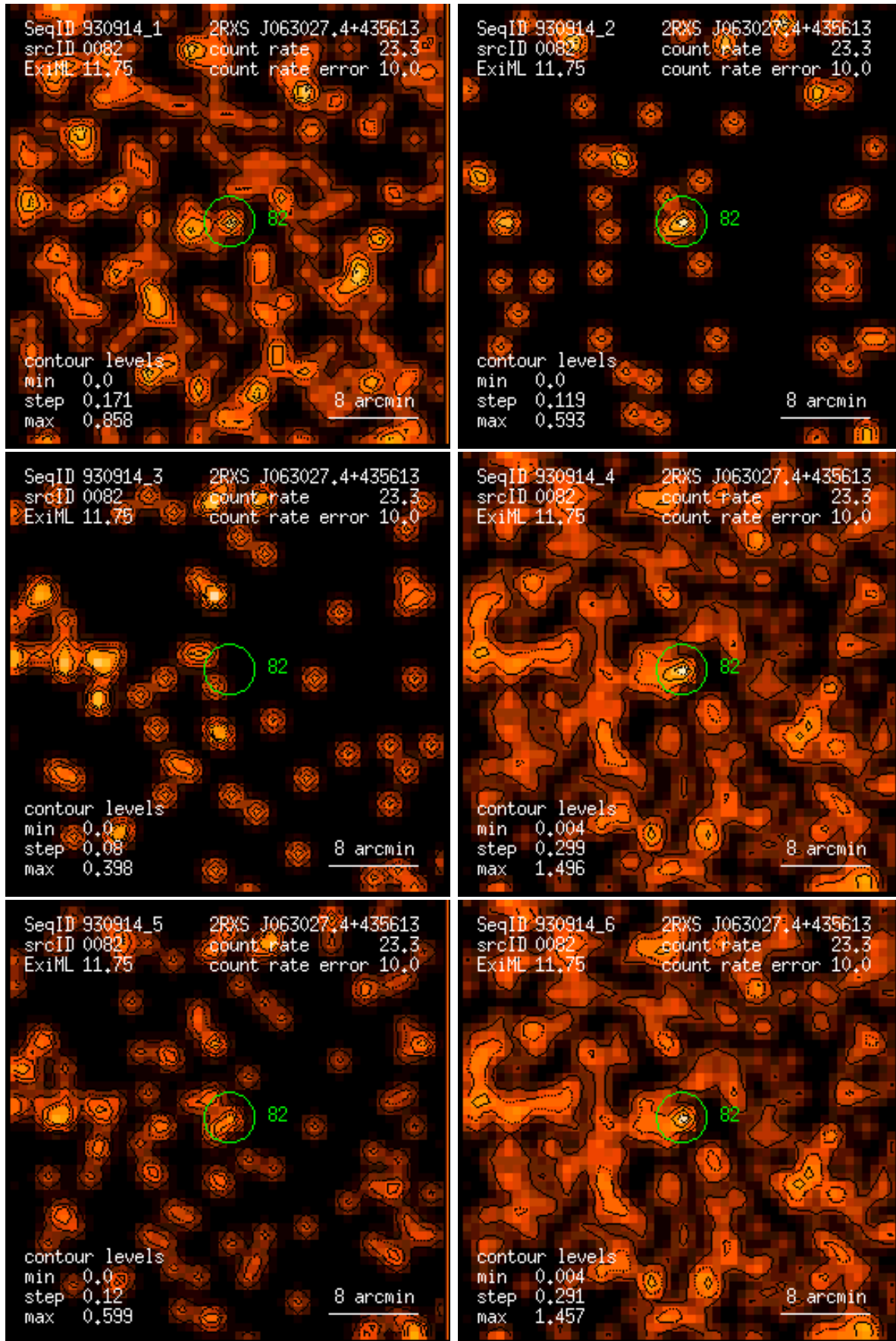
Figure 82: RASS 930914: detection 0082: band rate images, Gaussian filter: (1) PSPC channels 11 – 41, (2) 52 – 90, (3) 91 – 201, (4) 11 – 235, (5) 52 – 201, (6) 11 – 201. Broad band rates in counts/ks. Band rate contour levels in counts/ks/arcmin 2 .
