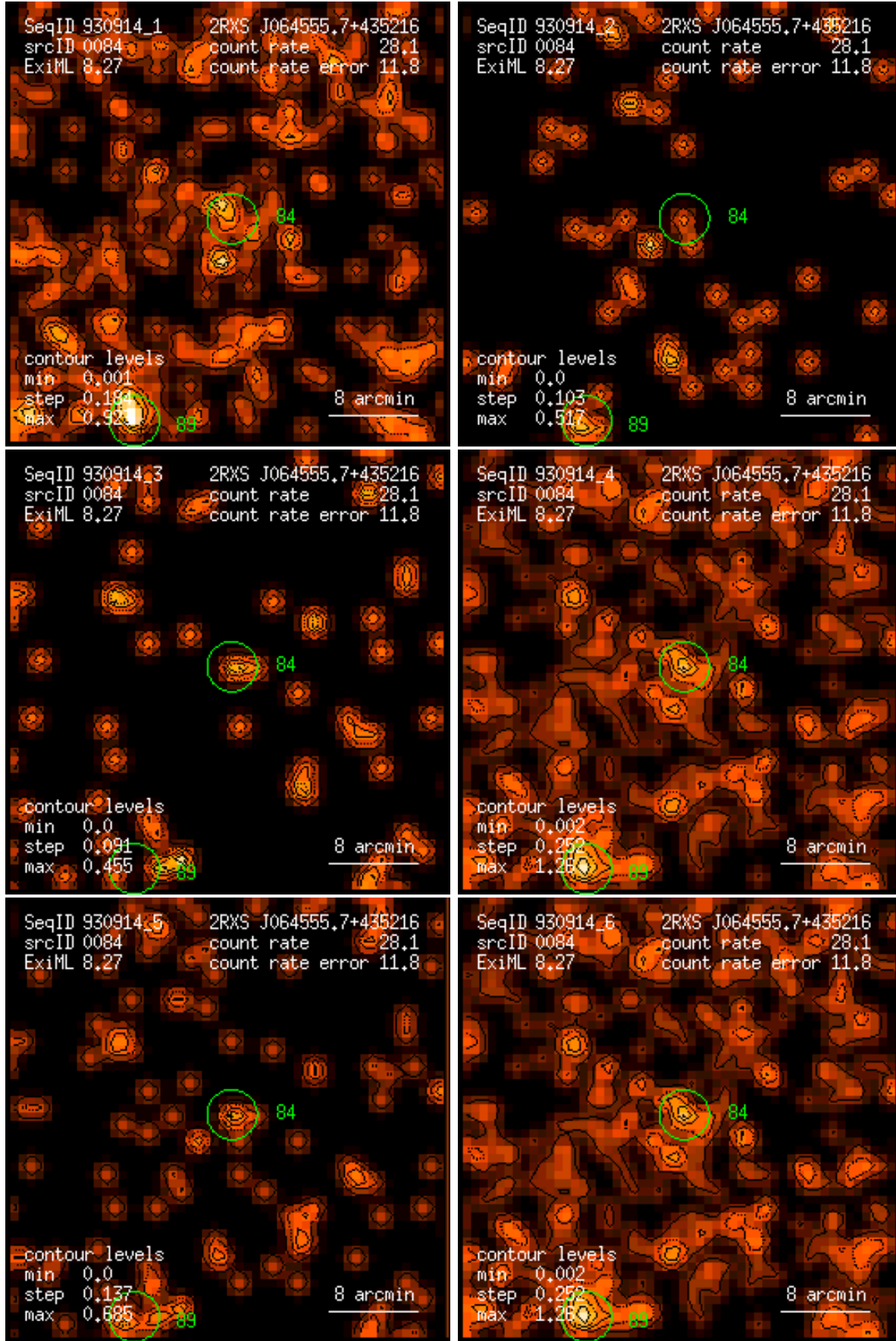
Figure 84: RASS 930914: detection 0084: band rate images, Gaussian filter: (1) PSPC channels 11 – 41, (2) 52 – 90, (3) 91 – 201, (4) 11 – 235, (5) 52 – 201, (6) 11 – 201. Broad band rates in counts/ks. Band rate contour levels in counts/ks/arcmin 2 .
