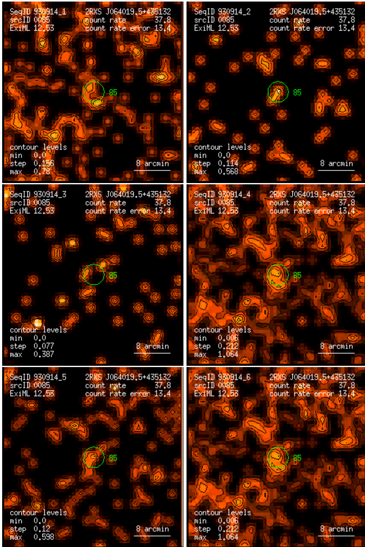
Figure 85: RASS 930914: detection 0085: band rate images, Gaussian filter: (1) PSPC channels 11 – 41, (2) 52 – 90, (3) 91 – 201, (4) 11 – 235, (5) 52 – 201, (6) 11 – 201. Broad band rates in counts/ks. Band rate contour levels in counts/ks/arcmin 2 .
