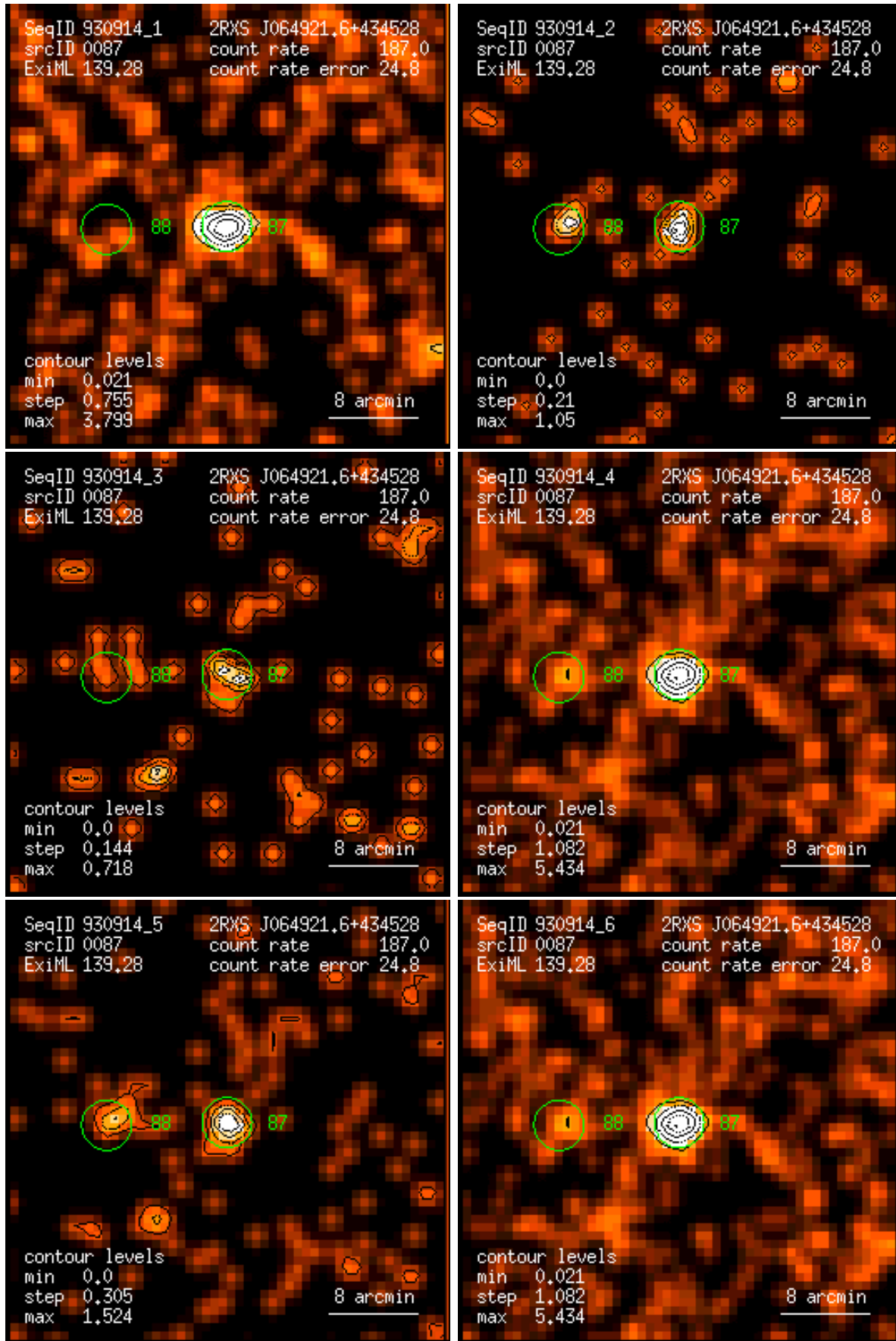
Figure 87: RASS 930914: detection 0087: band rate images, Gaussian filter: (1) PSPC channels 11 – 41, (2) 52 – 90, (3) 91 – 201, (4) 11 – 235, (5) 52 – 201, (6) 11 – 201. Broad band rates in counts/ks. Band rate contour levels in counts/ks/arcmin 2 .
