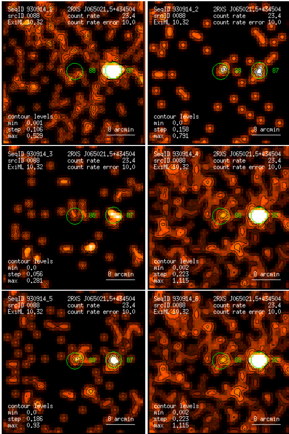
Figure 88: RASS 930914: detection 0088: band rate images, Gaussian filter: (1) PSPC channels 11 – 41, (2) 52 – 90, (3) 91 – 201, (4) 11 – 235, (5) 52 – 201, (6) 11 – 201. Broad band rates in counts/ks. Band rate contour levels in counts/ks/arcmin 2 .
