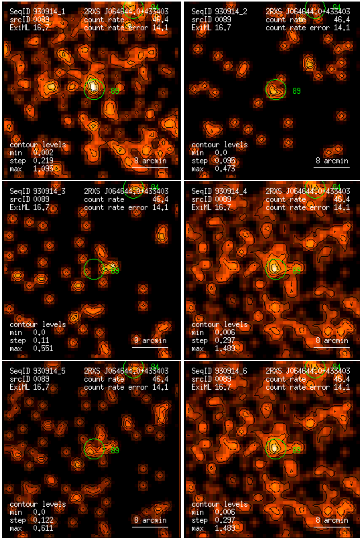
Figure 89: RASS 930914: detection 0089: band rate images, Gaussian filter: (1) PSPC channels 11 – 41, (2) 52 – 90, (3) 91 – 201, (4) 11 – 235, (5) 52 – 201, (6) 11 – 201. Broad band rates in counts/ks. Band rate contour levels in counts/ks/arcmin 2 .
