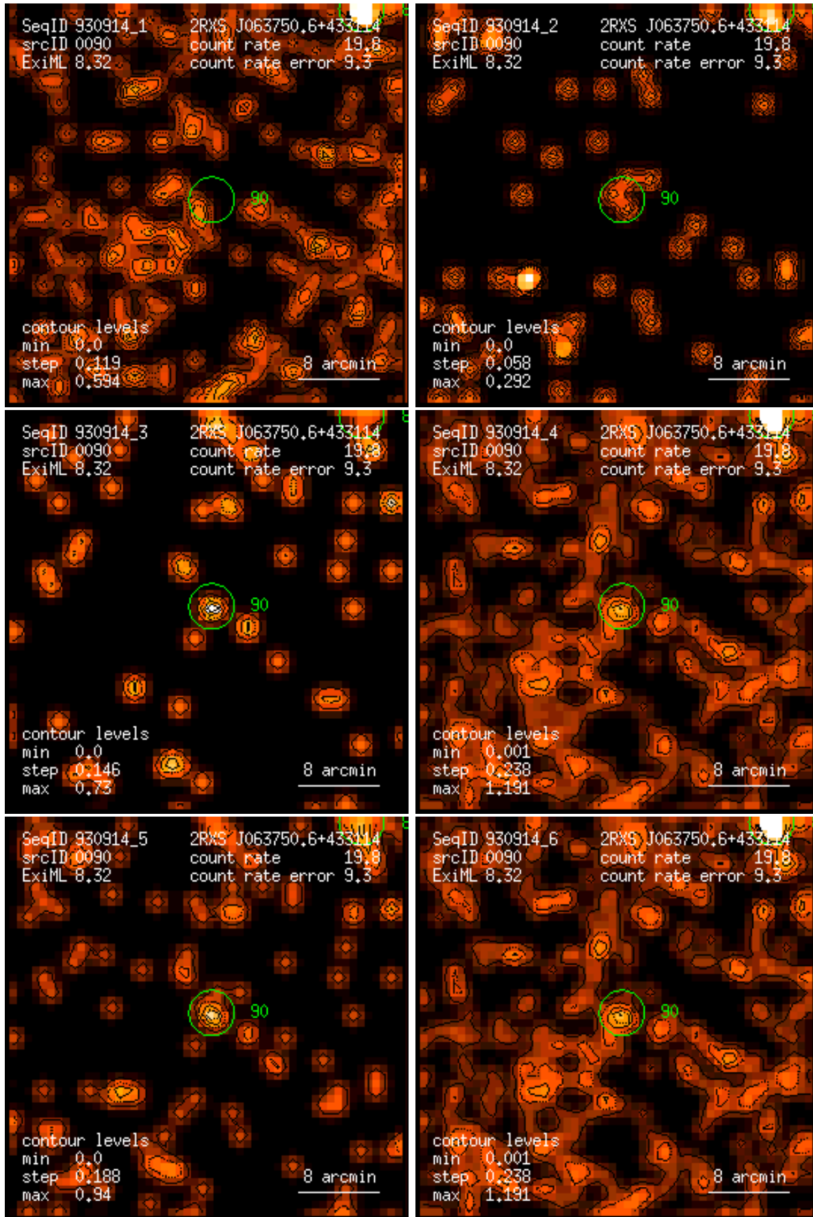
Figure 90: RASS 930914: detection 0090: band rate images, Gaussian filter: (1) PSPC channels 11 – 41, (2) 52 – 90, (3) 91 – 201, (4) 11 – 235, (5) 52 – 201, (6) 11 – 201. Broad band rates in counts/ks. Band rate contour levels in counts/ks/arcmin 2 .
