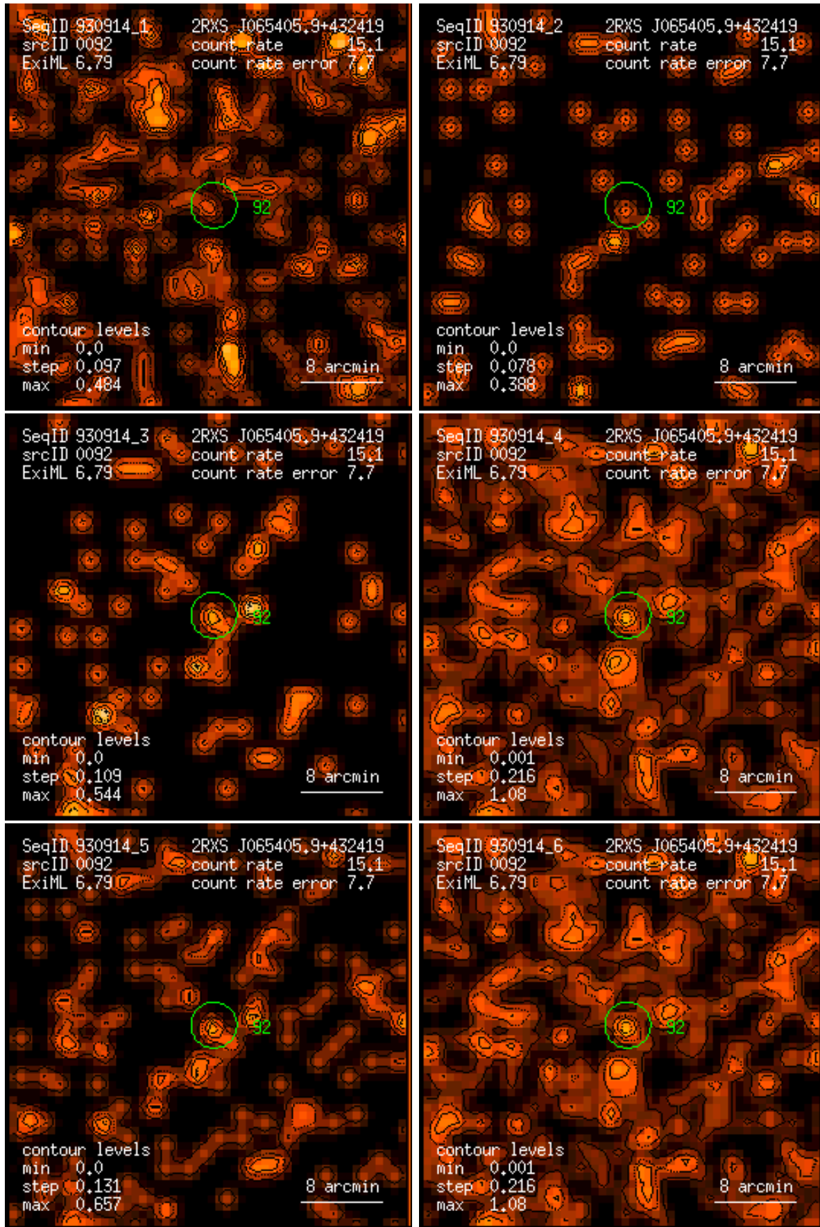
Figure 92: RASS 930914: detection 0092: band rate images, Gaussian filter: (1) PSPC channels 11 – 41, (2) 52 – 90, (3) 91 – 201, (4) 11 – 235, (5) 52 – 201, (6) 11 – 201. Broad band rates in counts/ks. Band rate contour levels in counts/ks/arcmin 2 .
