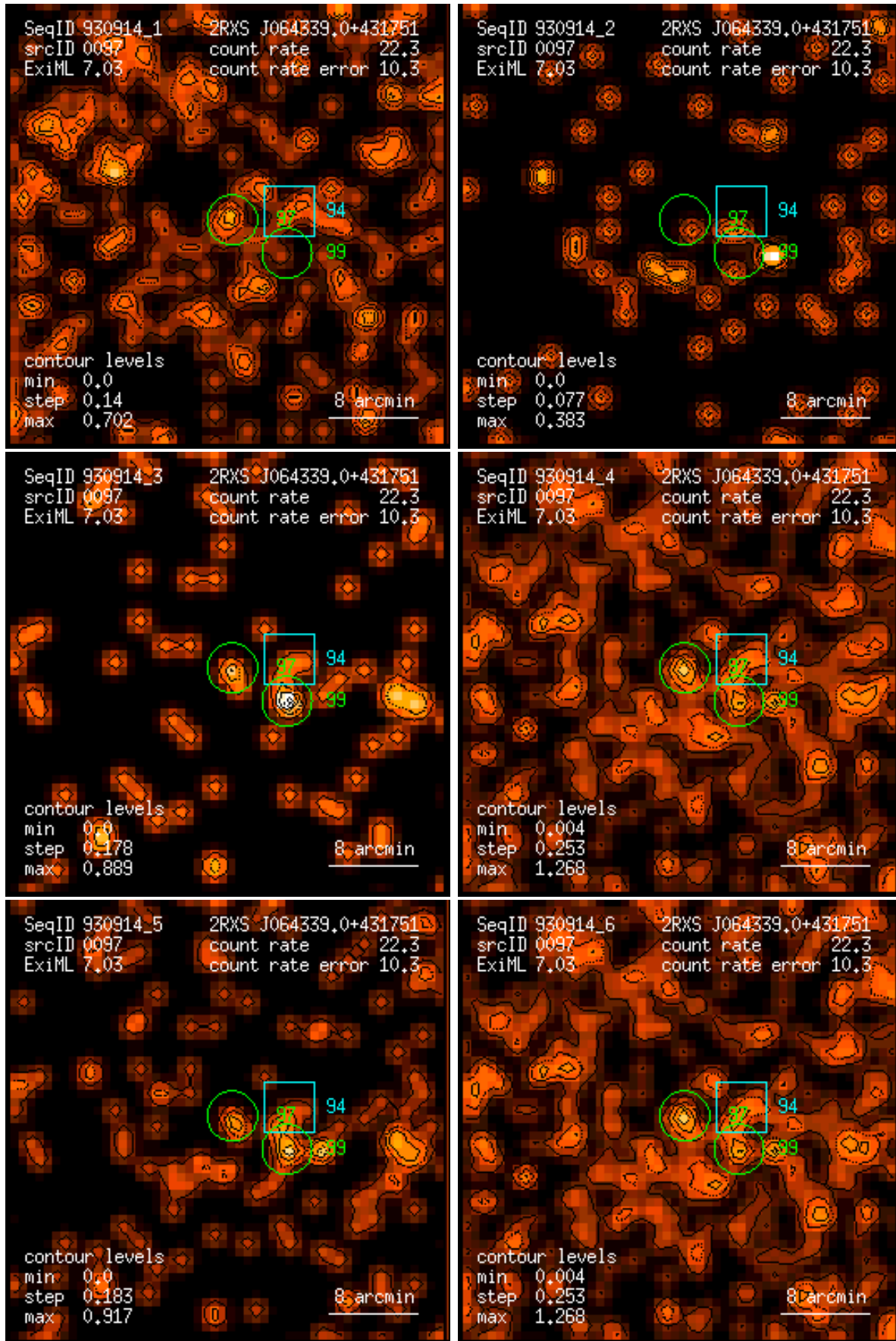
Figure 97: RASS 930914: detection 0097: band rate images, Gaussian filter: (1) PSPC channels 11 – 41, (2) 52 – 90, (3) 91 – 201, (4) 11 – 235, (5) 52 – 201, (6) 11 – 201. Broad band rates in counts/ks. Band rate contour levels in counts/ks/arcmin 2 .
