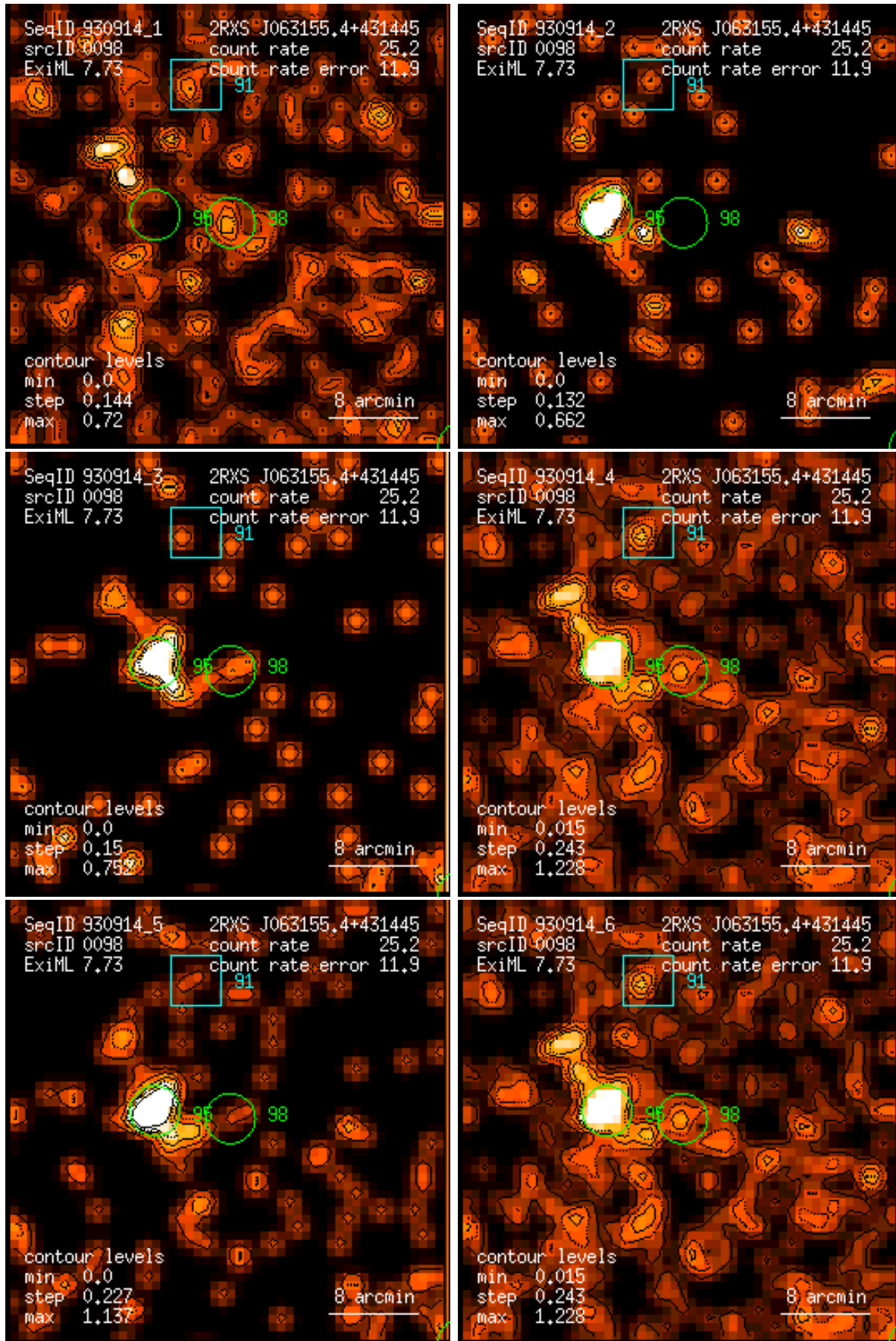
Figure 98: RASS 930914: detection 0098: band rate images, Gaussian filter: (1) PSPC channels 11 – 41, (2) 52 – 90, (3) 91 – 201, (4) 11 – 235, (5) 52 – 201, (6) 11 – 201. Broad band rates in counts/ks. Band rate contour levels in counts/ks/arcmin 2 .
