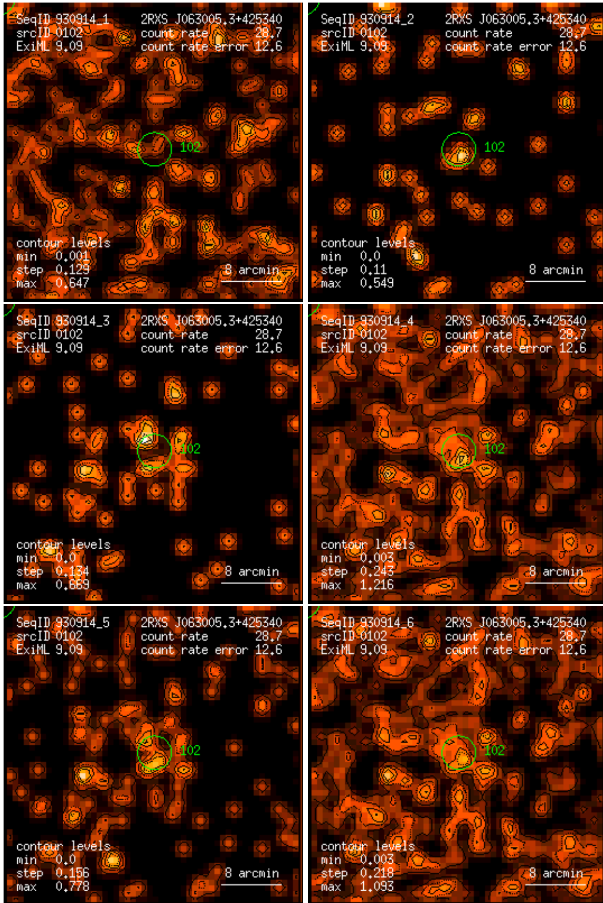
Figure 102: RASS 930914: detection 0102: band rate images, Gaussian filter: (1) PSPC channels 11 – 41, (2) 52 – 90, (3) 91 – 201, (4) 11 – 235, (5) 52 – 201, (6) 11 – 201. Broad band rates in counts/ks. Band rate contour levels in counts/ks/arcmin 2 .
